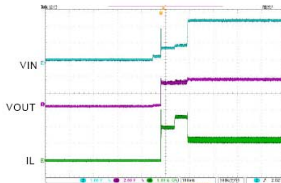
6. Start-Up Waveform
