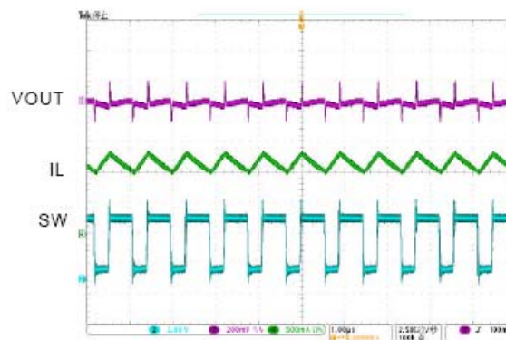
8. Switching Waveform
