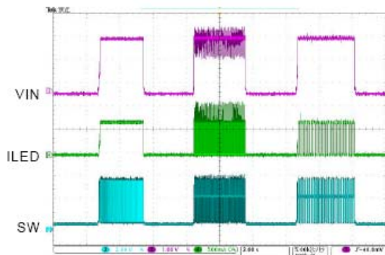
5. 3 Modes Change
