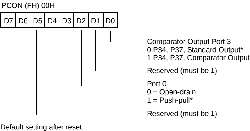
Figure 20. Port Configuration Register (PCON)—(0F) 0H: Write Only
