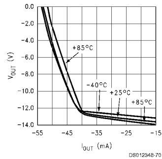
Output Voltage vs Output Current ( I_{SINK} , V_S = \pm 15\text{V} )
