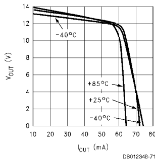
Output Voltage vs Output Current ( I_{SOURCE} , V_S = \pm 15\text{V} )
