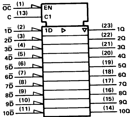
'ALS29842 logic symbol†
