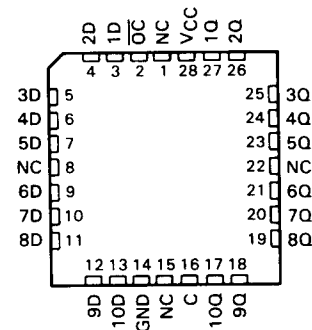
SN74ALS29842 . . . DW OR NT PACKAGE (TOP VIEW)
