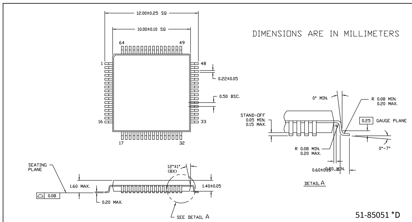
Figure 8 64-pin TQFP package (0.5-mm pitch) outline
