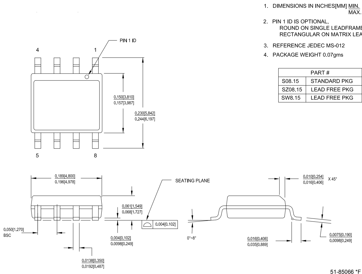
Figure 12. 8-pin (150-mil) SOIC Package Outline
