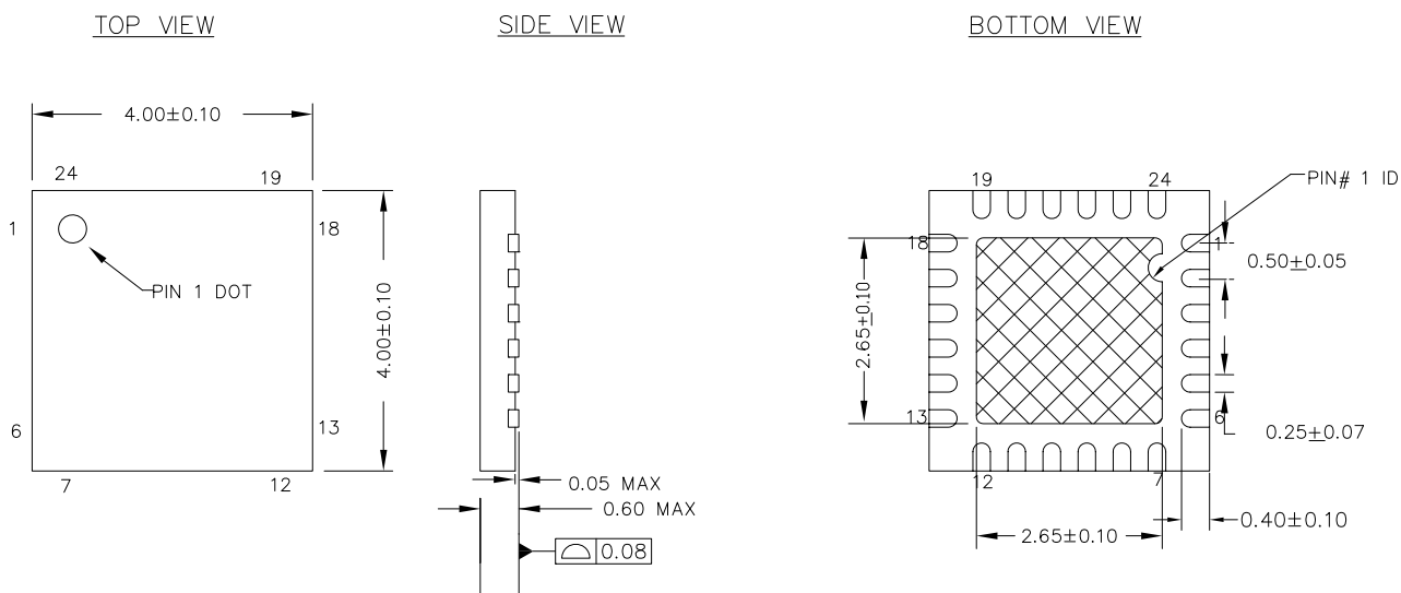
Figure 9. 24-pin QFN EPAD (Sawn) Package Outline
