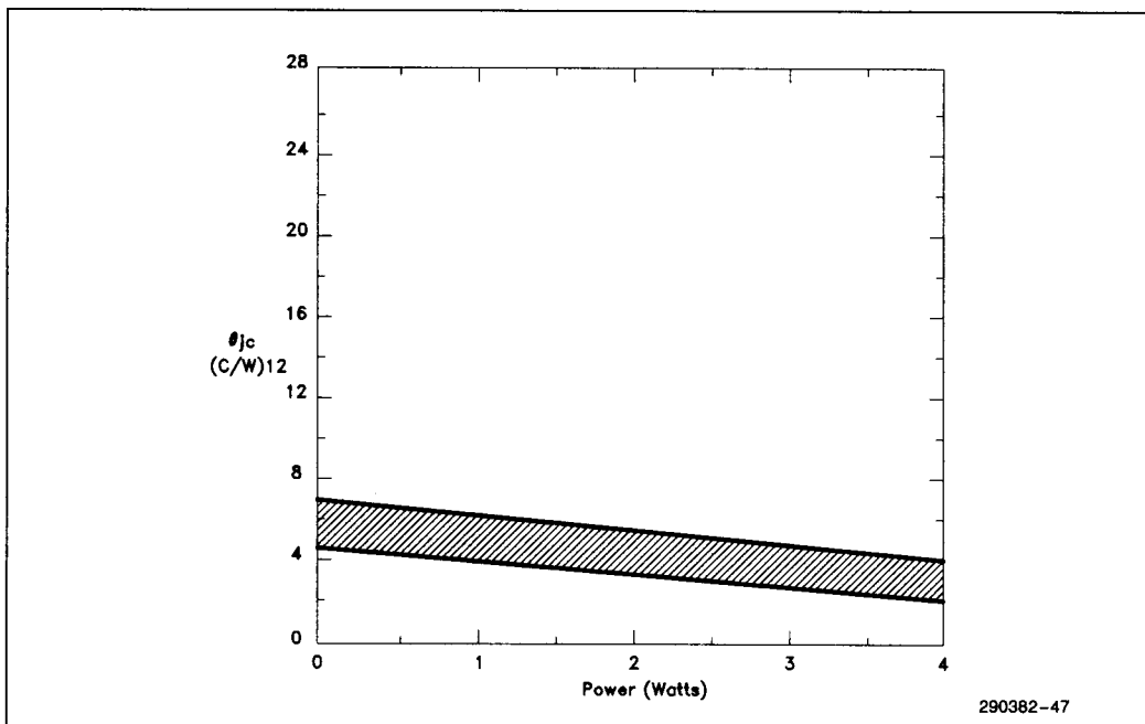
Figure 8.5 - Junction to Case Thermal Resistance vs Power
