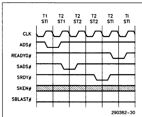
Figure 6.6 - I/O Read Cycle
