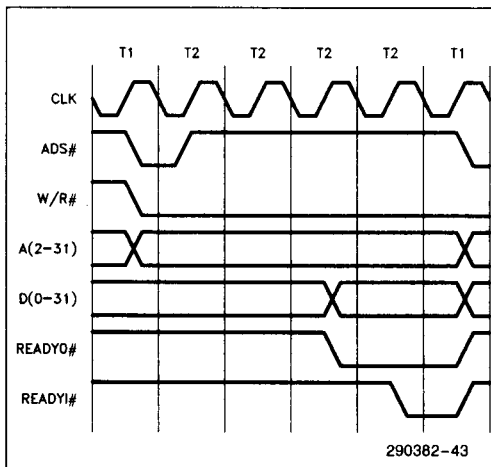
Figure 7.1 - SRAM Mode Read Cycle
