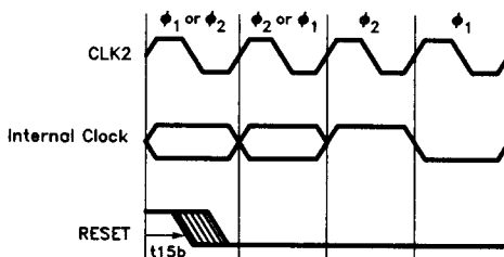
Figure 3.2 - RESET/Internal Phase Relationship
