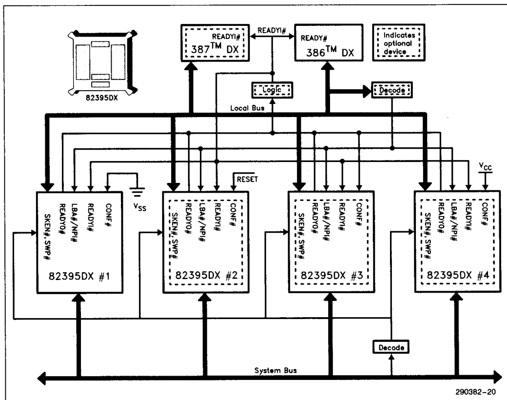
Figure 4.6 - System Description
