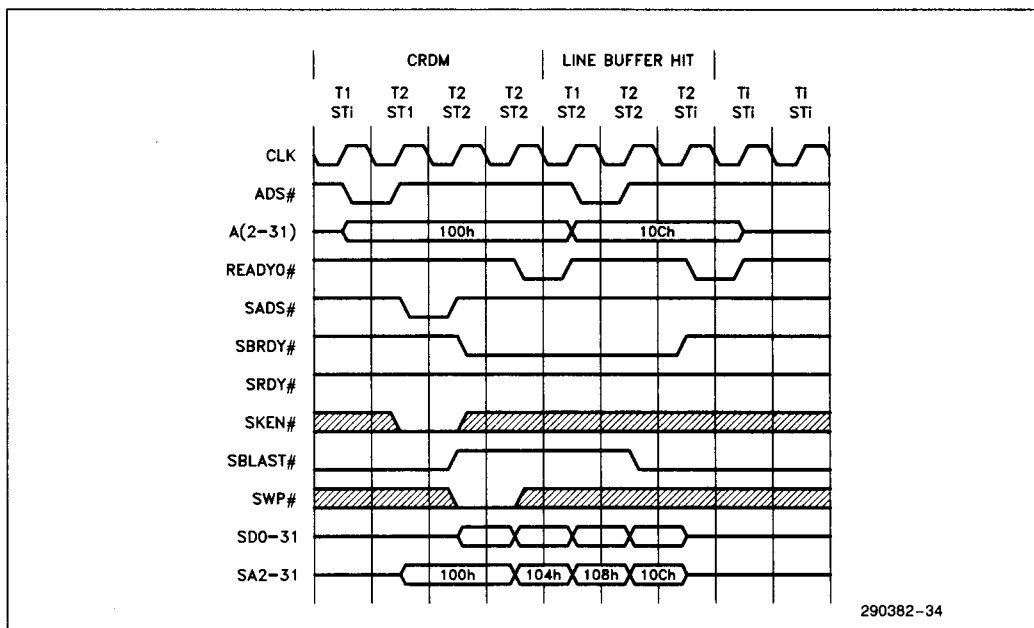
Figure 6.9 - Line Fill Without Burst or Pipeline
