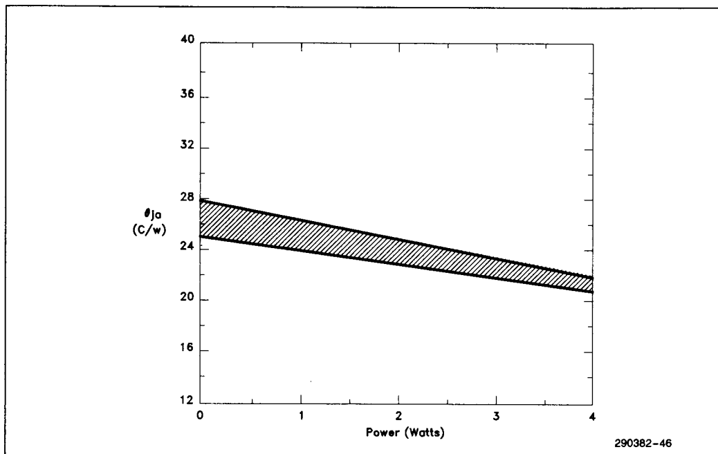
Figure 8.4 - Junction to Ambient Thermal Resistance vs Power
