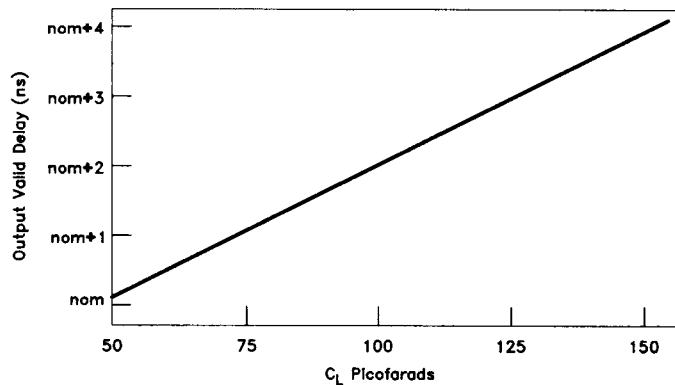
Figure 9.6 - Typical Output Valid Delay vs Load Capacitance at Maximum Operating Temperature ( C_L = 50\text{pF} )
