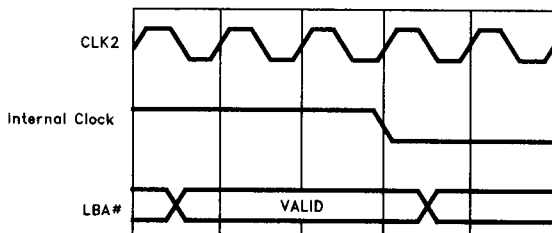
Figure 3.3 - Sampling LBA# During RESET
