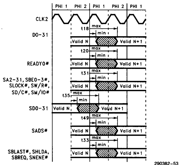
Figure 9.4 - AC Timing Waveforms - Output Valid Delay
