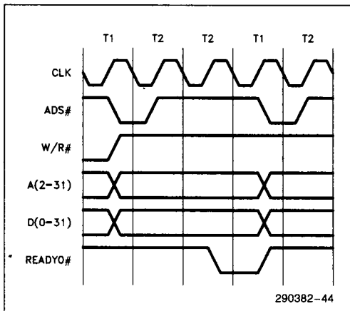
Figure 7.2 - SRAM Mode Write Cycle
