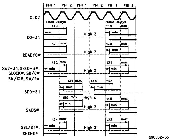
Figure 9.5 - AC Timing Waveforms - Output Float Delays
