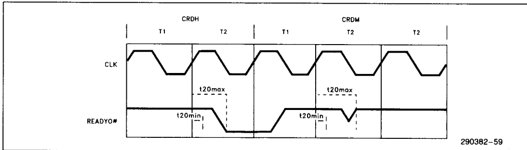
Figure 4.0 READYO# Behavior
