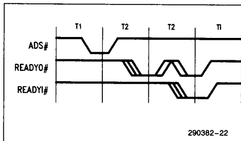
Figure 5.2 - Externally Delayed READY
