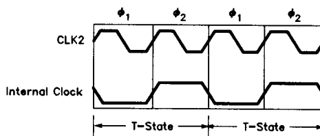
Figure 3.1 - CLK2 and Internal Clock
