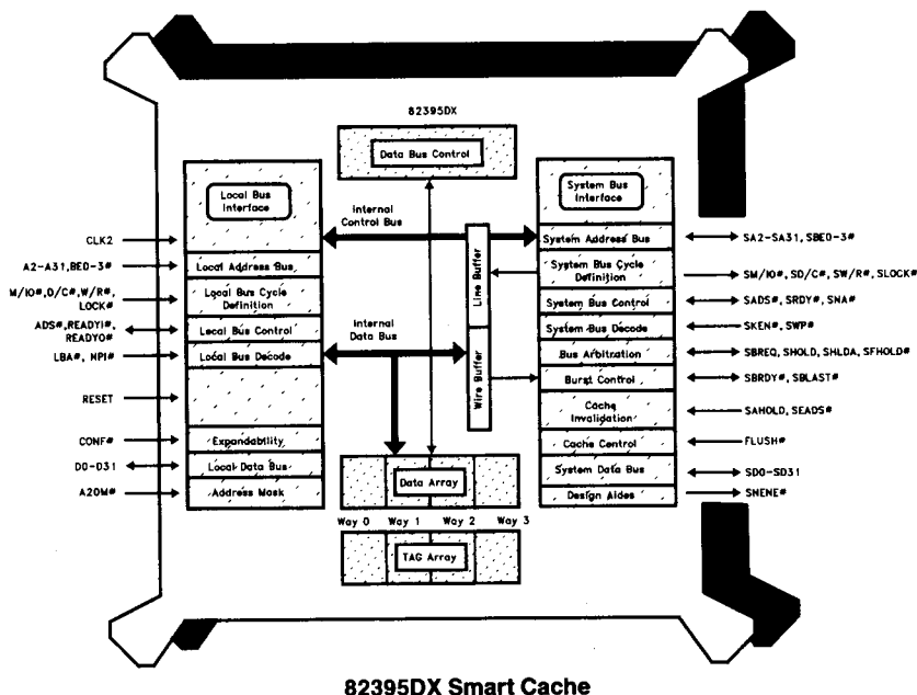
82395DX Smart Cache
