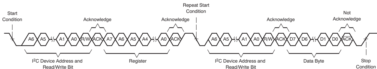
Figure 82. I 2 C Single-Byte Read Transfer
