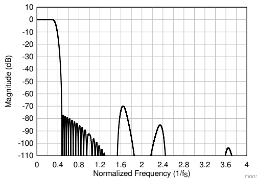
Figure 47. Linear Phase Decimation Filter Magnitude Response
