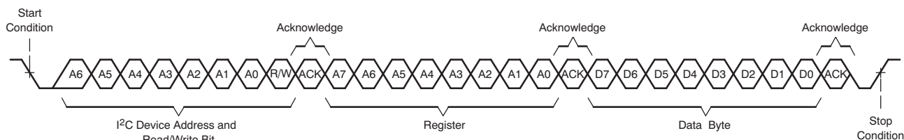
Figure 80. I²C Single-Byte Write Transfer
