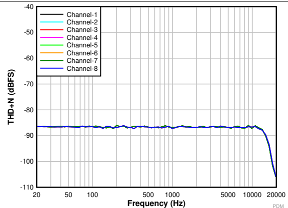
Fourth order PDM modulator with PDMCLKx = 1.536\text{ MHz}
