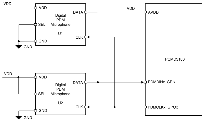
Figure 30. Digital PDM Microphones Connection Diagram to the PCMD3180
