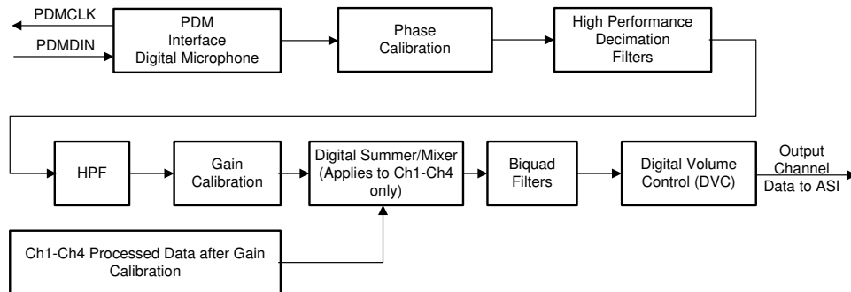
Figure 32. Signal-Chain Processing Flowchart
