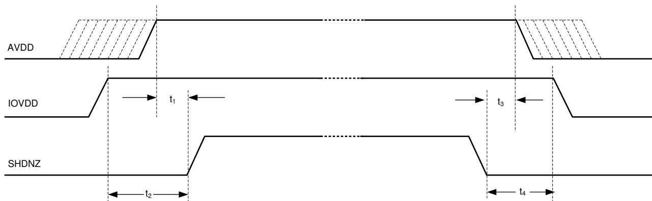
Figure 164. Power-Supply Sequencing Requirement Timing Diagram
