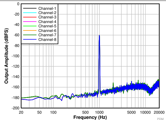
Fifth order PDM modulator with PDMCLKx = 3.072\text{ MHz}
