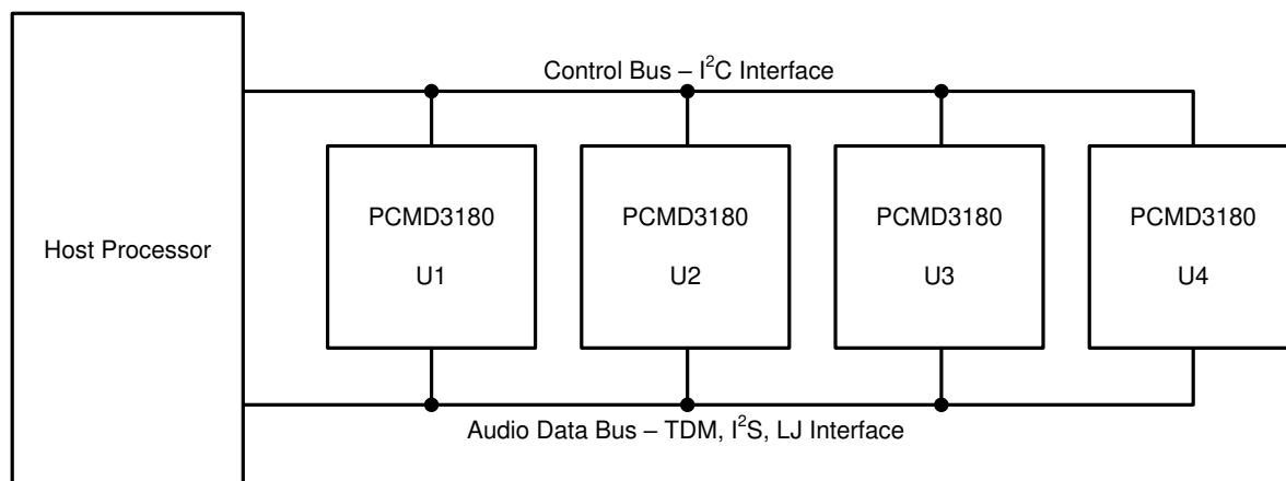
Figure 29. Multiple PCMD3180 Devices With Shared Control and Audio Data Buses
