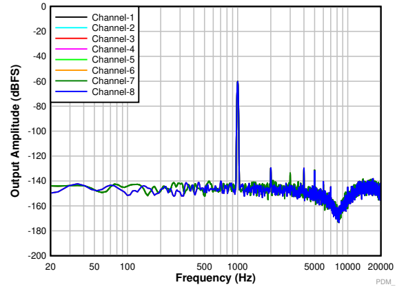
Fourth order PDM modulator with PDMCLKx = 3.072\text{ MHz}
