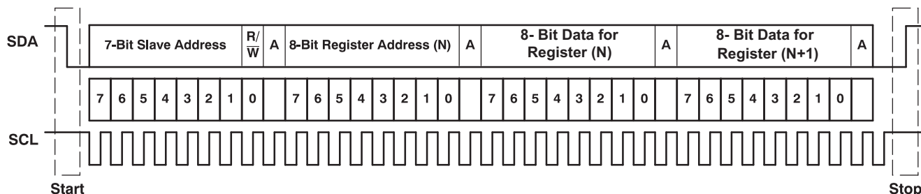
Figure 79. Typical I²C Sequence
