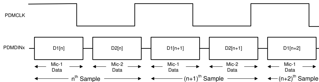
Figure 31. Digital PDM Microphone Protocol Timing Diagram
