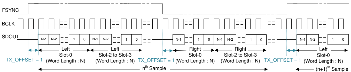
Figure 28. LJ Protocol Timing (TX_OFFSET = 1 and BCLK_POL = 1)
