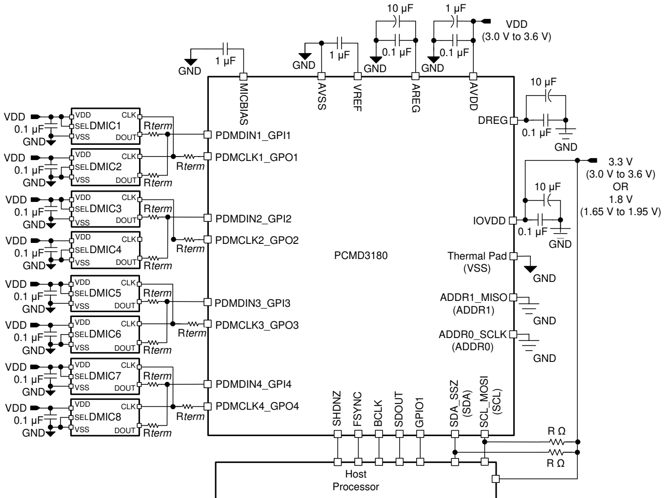
Figure 161. Eight-Channel Digital PDM Microphone Recording Diagram
