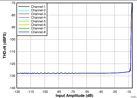
Fifth order PDM modulator with PDMCLKx = 3.072\text{ MHz}
