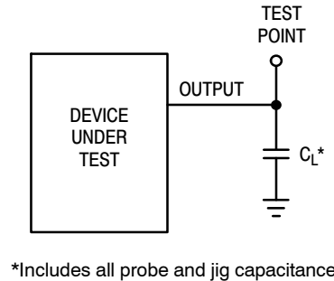
Figure 2. Test Circuit
