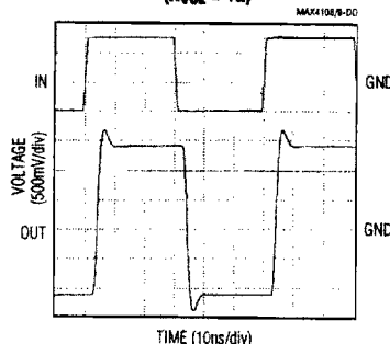
MAX4109 LARGE-SIGNAL PULSE RESPONSE ( A_{VCL} = +2 )
