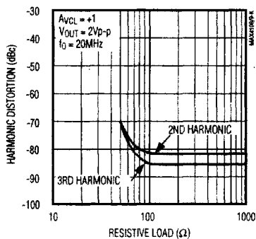
MAX4108 HARMONIC DISTORTION vs. LOAD
