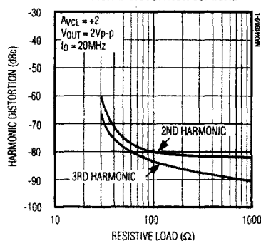
MAX4109 HARMONIC DISTORTION vs. LOAD
