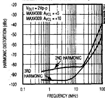
MAX4308/MAX4309 HARMONIC DISTORTION vs. FREQUENCY
