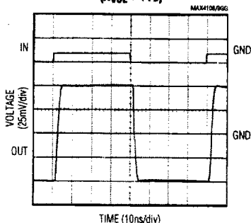
MAX4309 SMALL-SIGNAL PULSE RESPONSE ( A_{VCL} = +10 )
