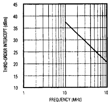
MAX4109 TWO-TONE THIRD-ORDER INTERCEPT vs. FREQUENCY
