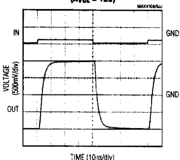
MAX4309 LARGE-SIGNAL PULSE RESPONSE ( A_{VCL} = +20 )
