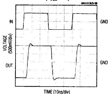
MAX4108 LARGE-SIGNAL PULSE RESPONSE ( A_{VCL} = +2 )
