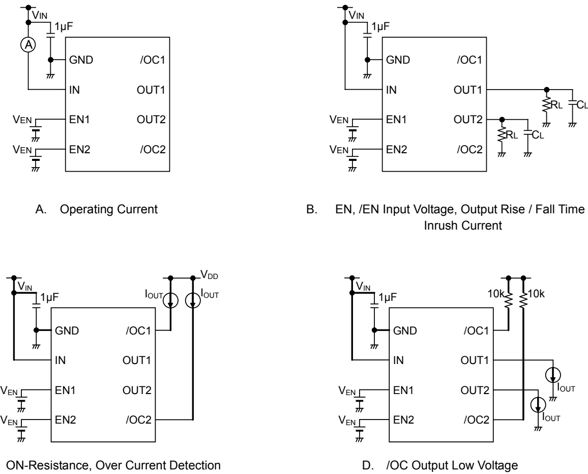
Figure 1. Measurement Circuit
