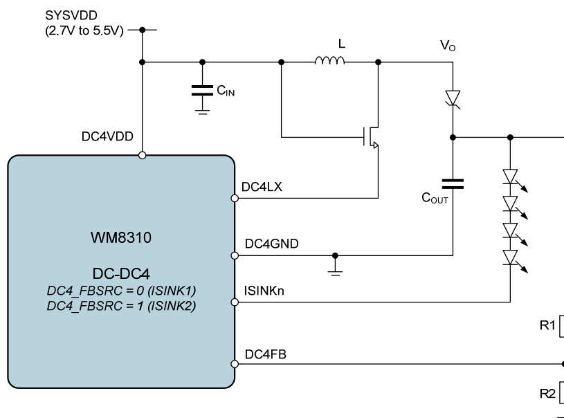
Figure 21 DC-DC Boost Converter Connections
