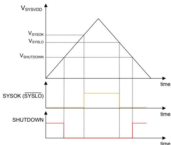
Figure 32 SYSVDD Monitoring
