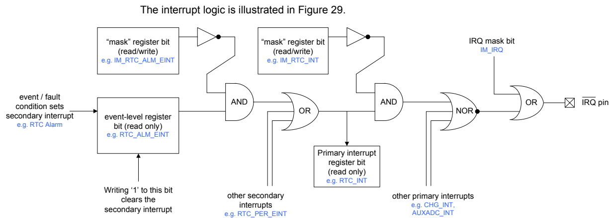
Figure 29 Interrupt Logic
