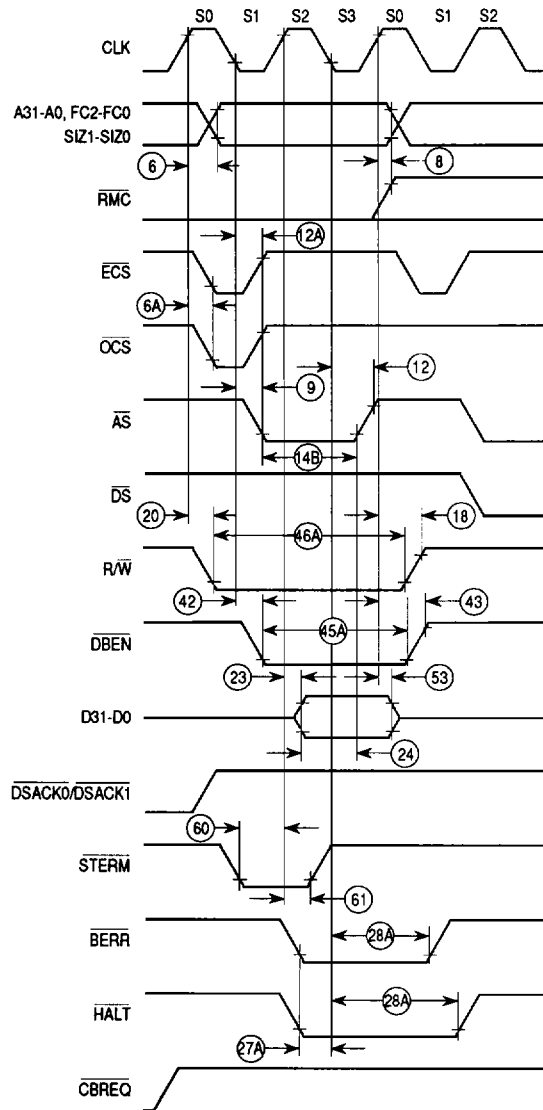
Figure 14. Synchronous Write Cycle Timing Diagram
