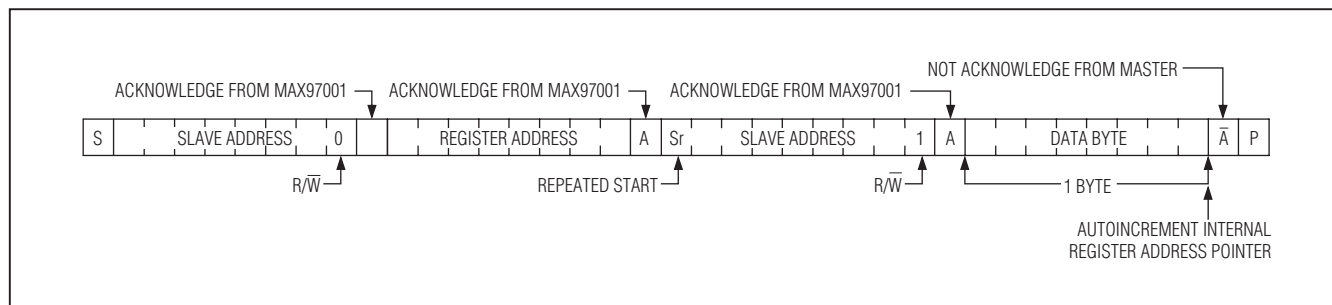
Figure 12. Reading One Byte of Data from the MAX97001
