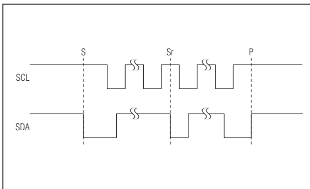
Figure 8. START, STOP, and REPEATED START Conditions
