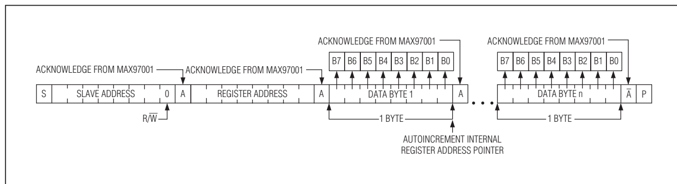
Figure 11. Writing n-Bytes of Data to the MAX97001
