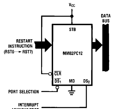
Interrupt Instruction Port
