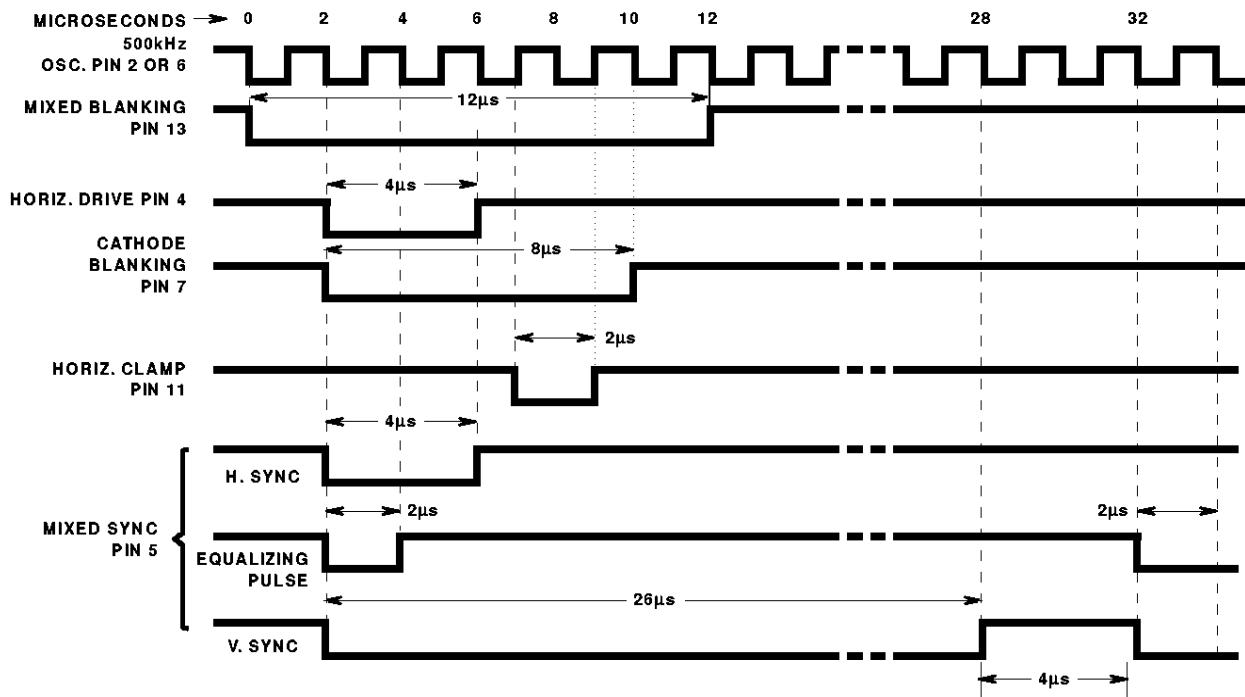
FIGURE 4. SYNC GENERATOR TIMING - 625/50Hz, HORIZONTAL TIMING WAVEFORMS
