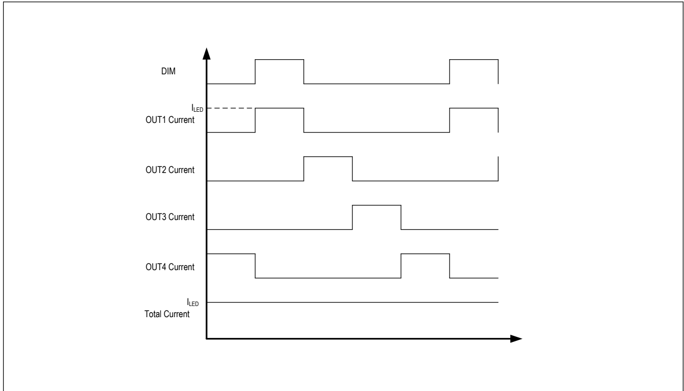
Figure 2. Phase-Shifted Outputs
