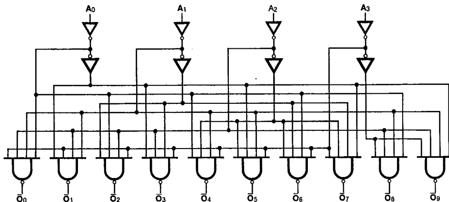
LOGIC DIAGRAM
