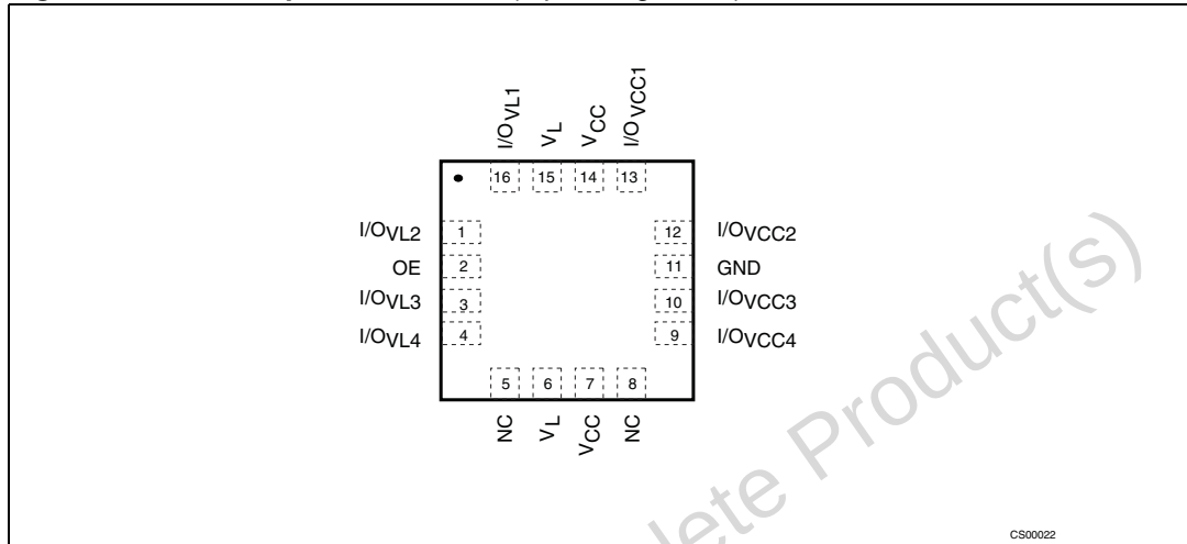
Figure 1. ST2349 pin connection (top through view)
