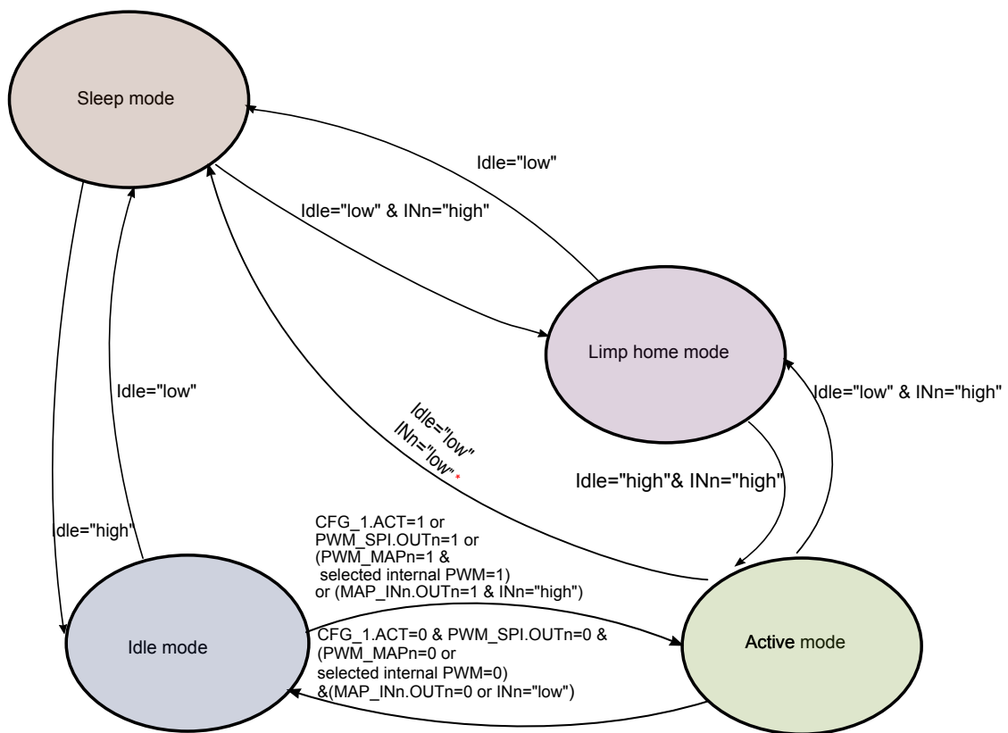
Figure 6. State diagram
