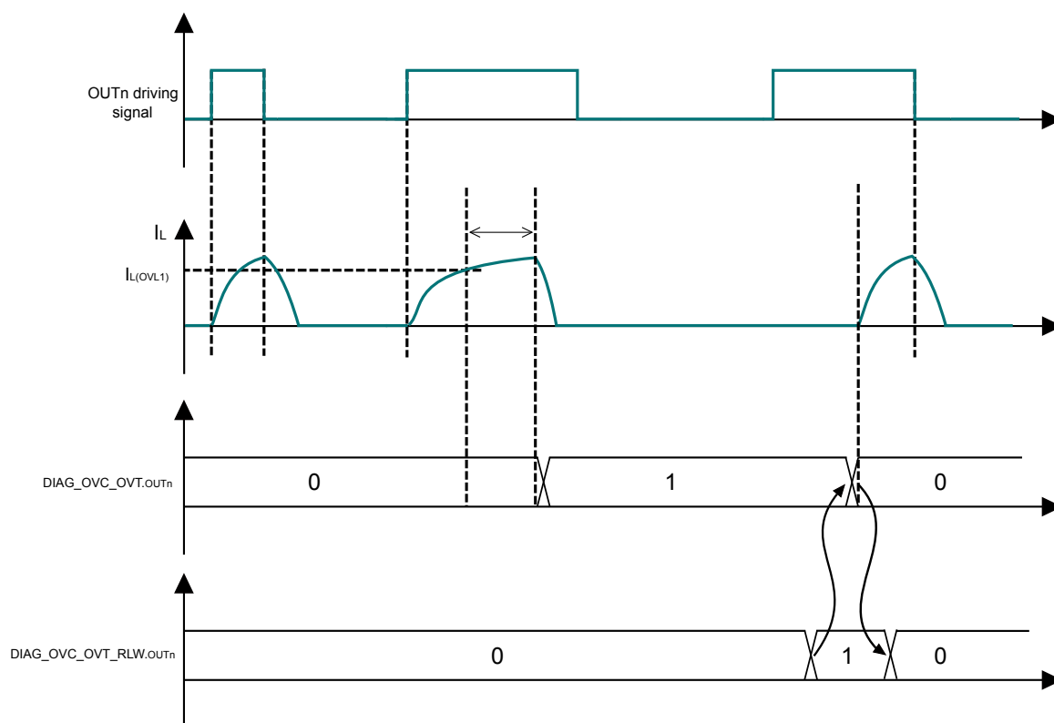
Figure 14. Latch off in overload condition
