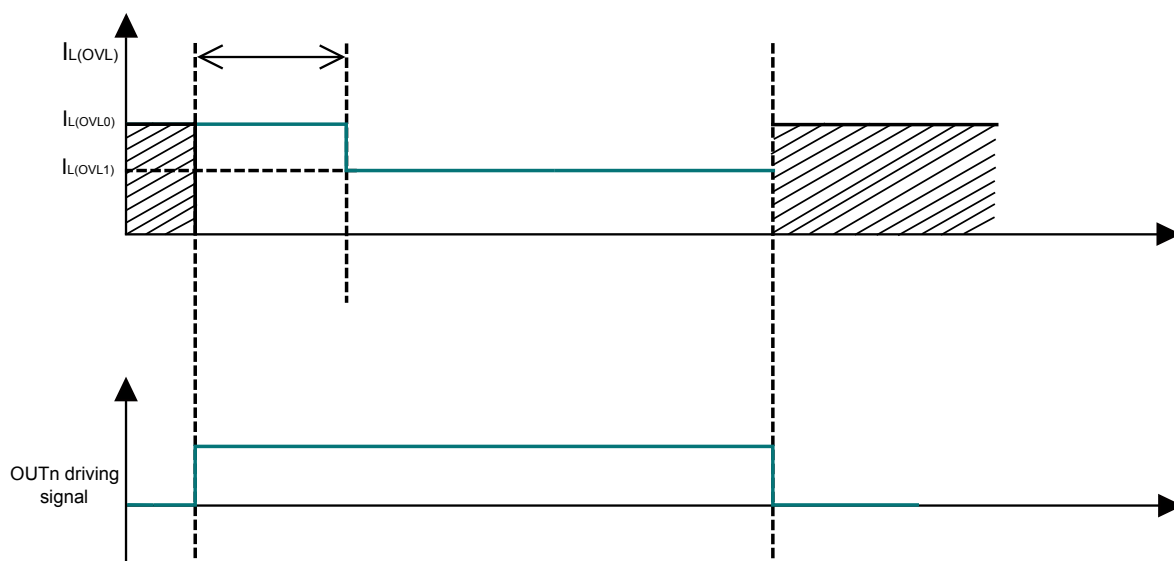
Figure 13. Overload thresholds
