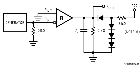
FIGURE 9. Receiver Propagation Delay Test Circuit
