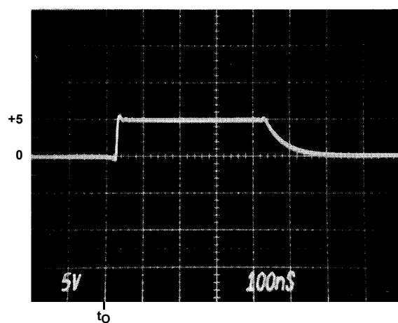
FIGURE 2C. V_{IN} = +5V
