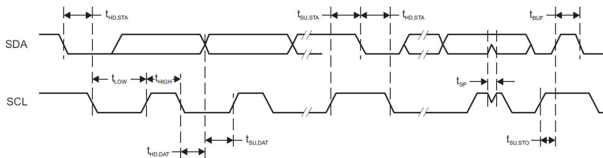
Figure 3.1 I²C Mode Timing
