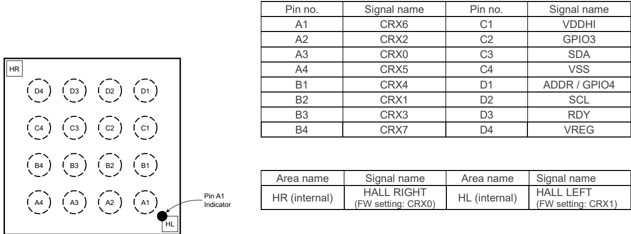
Figure 2.1 16-pin WLCSP Package (Top view)
