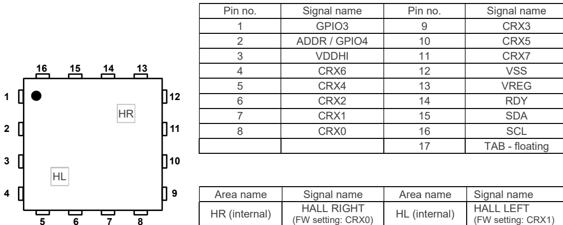
Figure 2.2 16-pin QFN Package (Top view)
