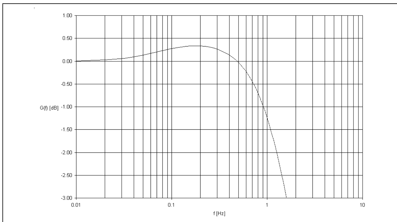
Figure 18 - Detailed DPLL Jitter Transfer Function Diagram
