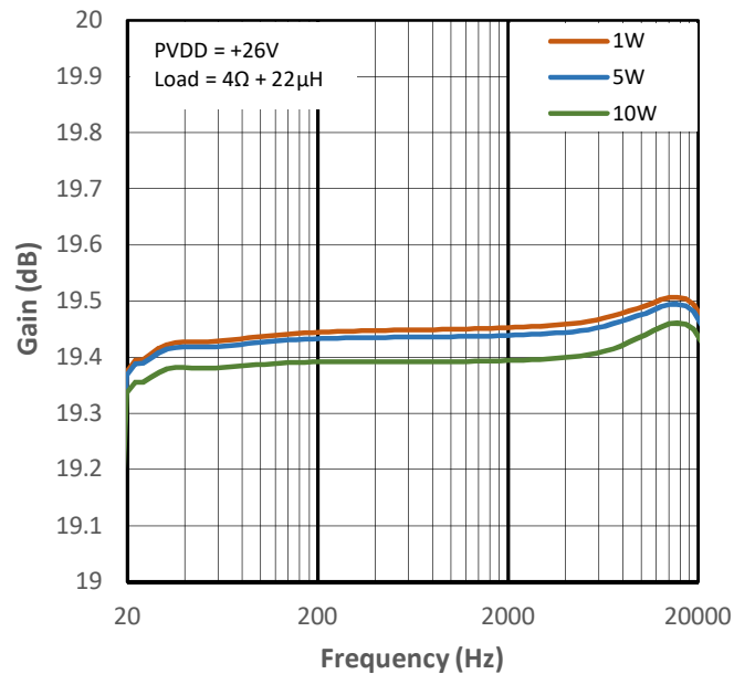
Figure 10-26 Low Gain vs Frequency for PMP1
