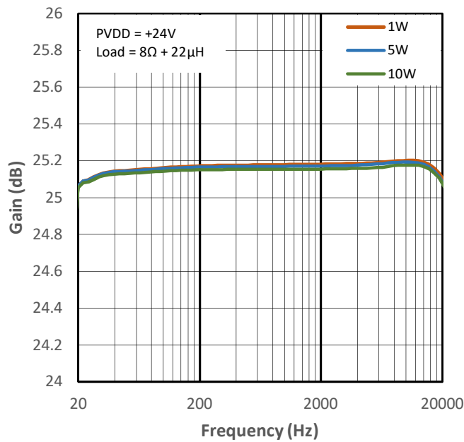
Figure 13-28 High Gain vs Frequency for PMP4
