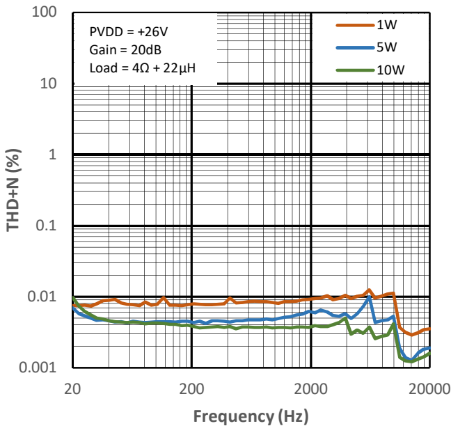
Figure 10-6 THD+N vs Frequency for PMP1
