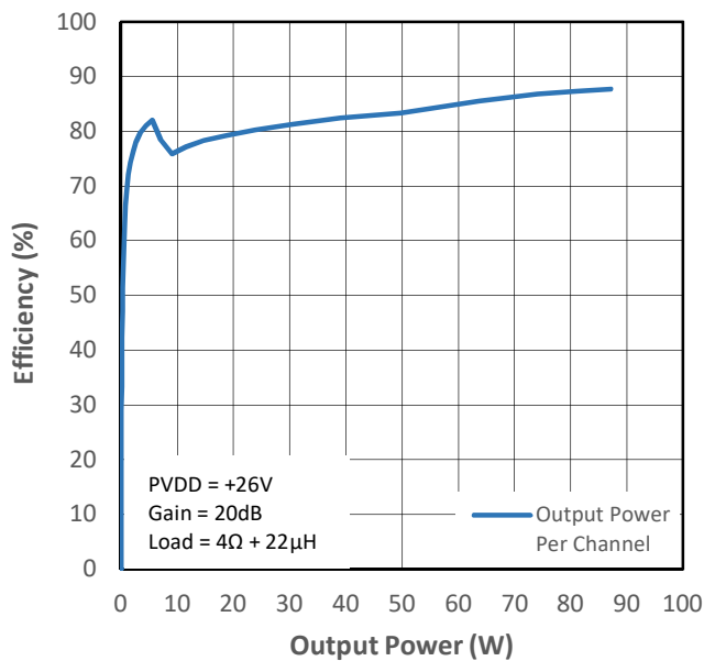
Figure 10-9 PMP0 Efficiency (VDD + PVDD) vs Output Power
