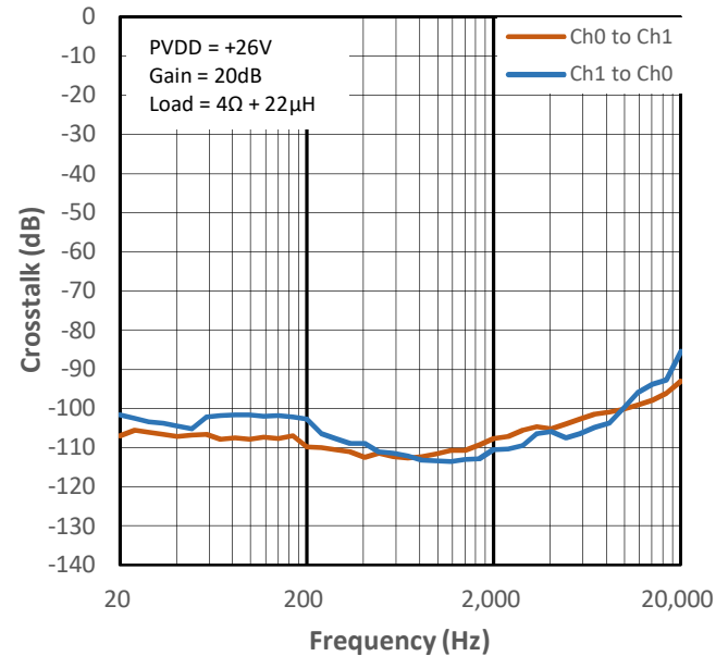
Figure 10-36 Crosstalk vs Frequency for PMP4
