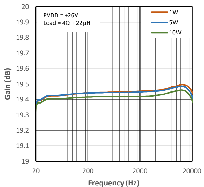
Figure 10-28 Low Gain vs Frequency for PMP4
