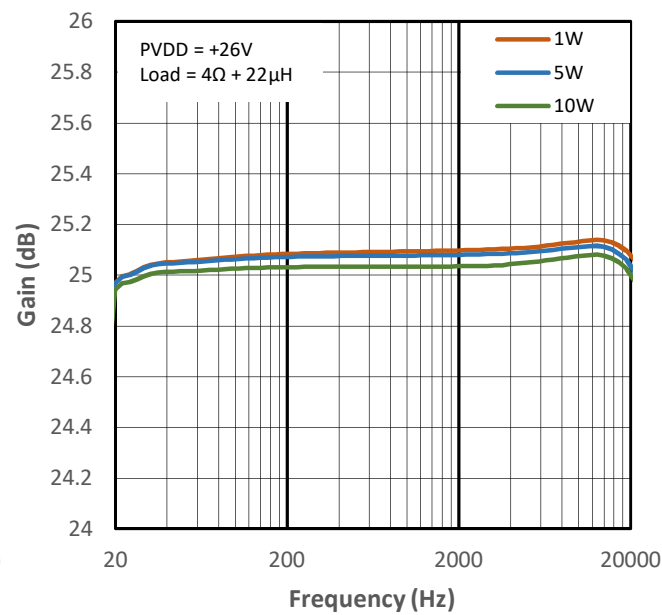
Figure 10-32 High Gain vs Frequency for PMP4
