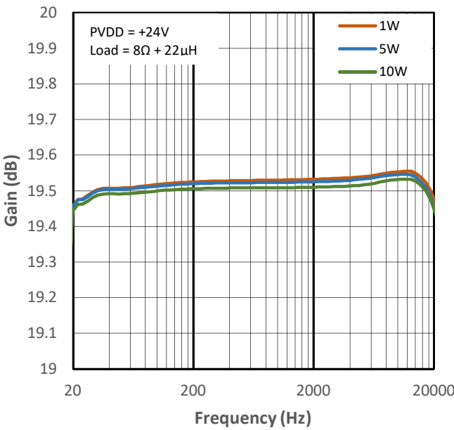
Figure 13-24 Low Gain vs Frequency for PMP4
