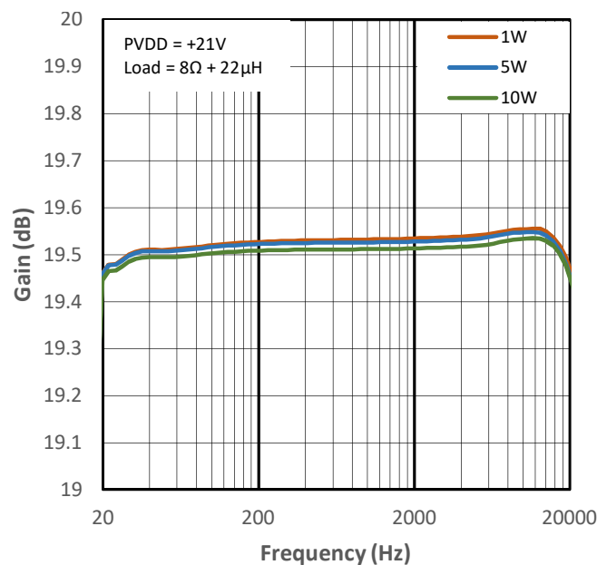
Figure 15-24 Low Gain vs Frequency for PMP4
