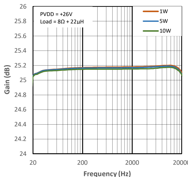
Figure 11-32 High Gain vs Frequency for PMP4
