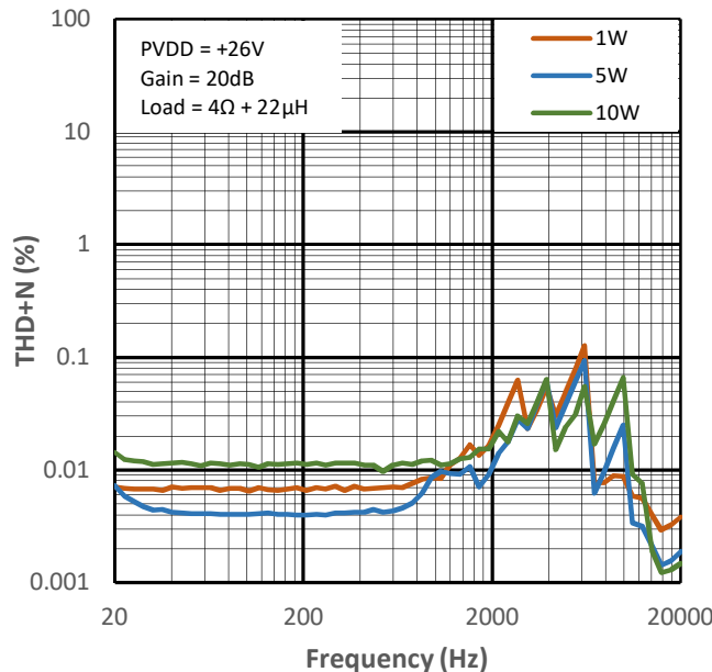
Figure 10-8 THD+N vs Frequency for PMP4
