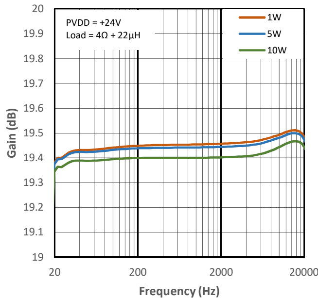
Figure 12-23 Low Gain vs Frequency for PMP2
