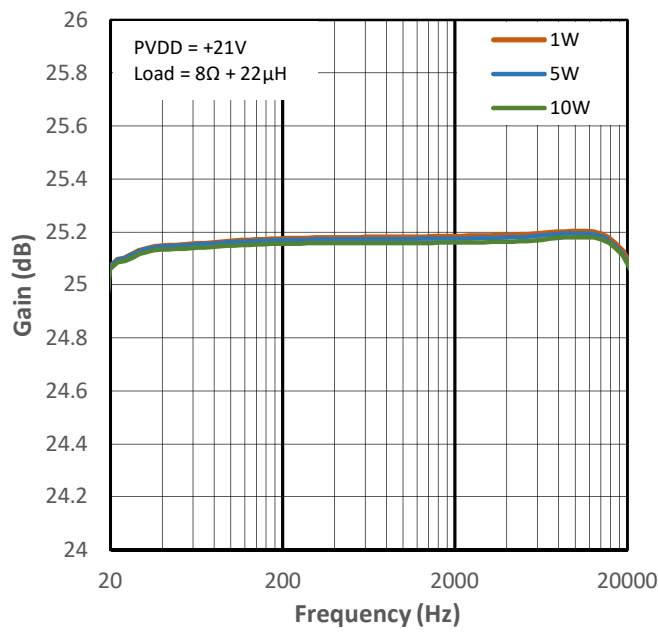
Figure 15-28 High Gain vs Frequency for PMP4
