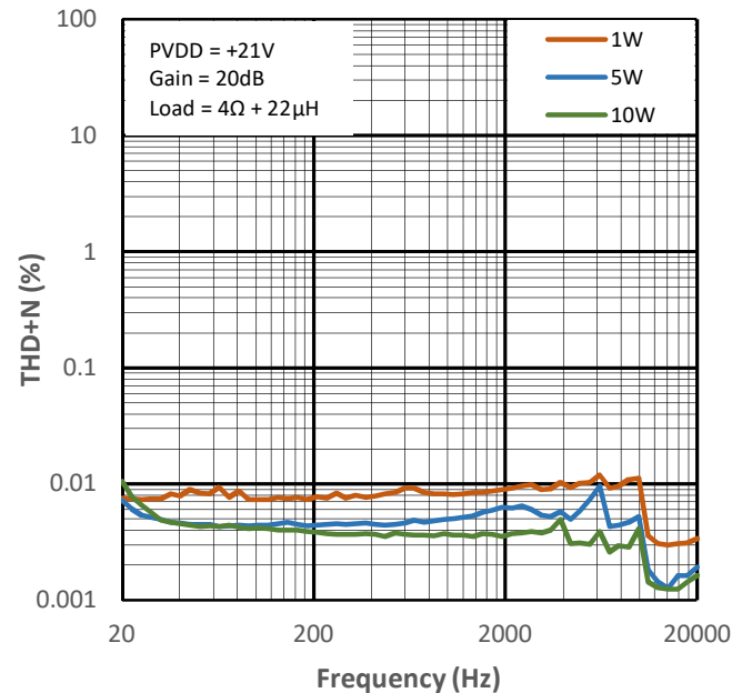
Figure 14-6 THD+N vs Frequency for PMP1
