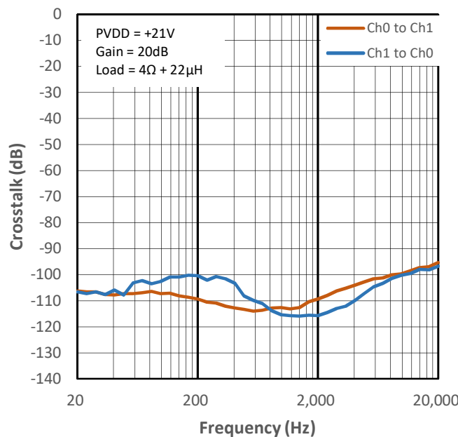
Figure 14-32 Crosstalk vs Frequency for PMP4
