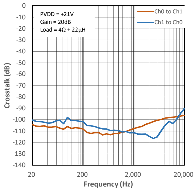
Figure 14-30 Crosstalk vs Frequency for PMP1
