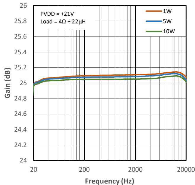
Figure 14-28 High Gain vs Frequency for PMP4
