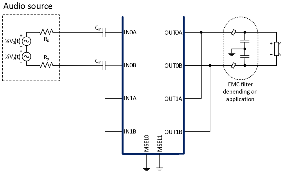
Figure 9-5 Parallel Bridge Tied Load (PBTB) configuration
