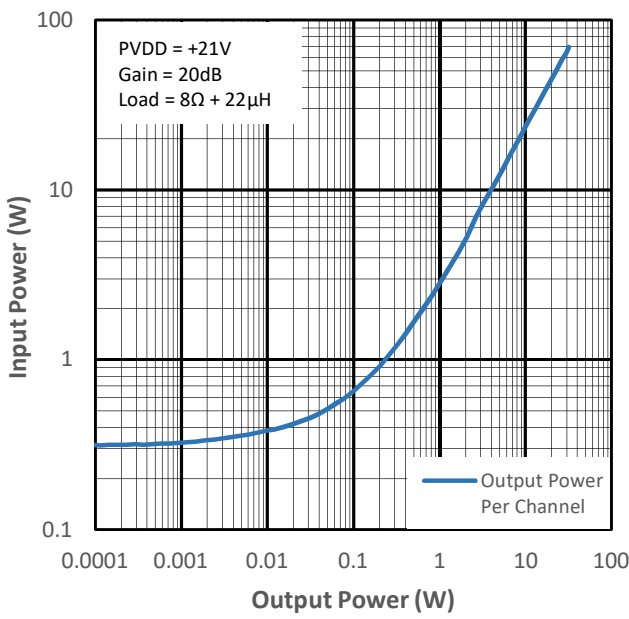
Figure 15-14 Input Power vs Output Power for PMP1
