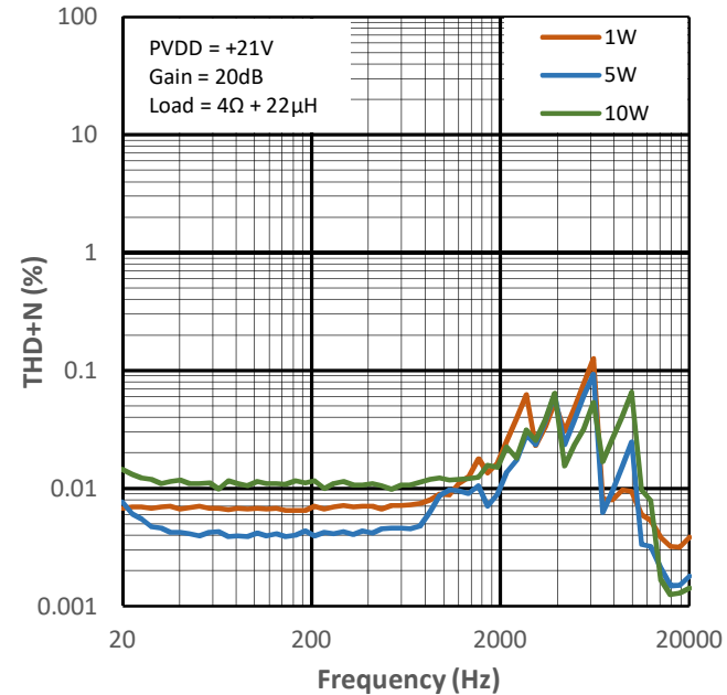
Figure 14-8 THD+N vs Frequency for PMP4
