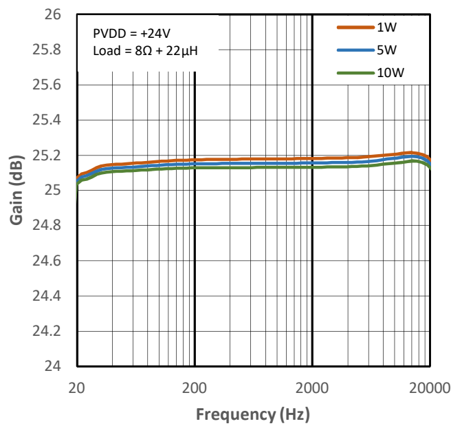
Figure 13-26 High Gain vs Frequency for PMP1
