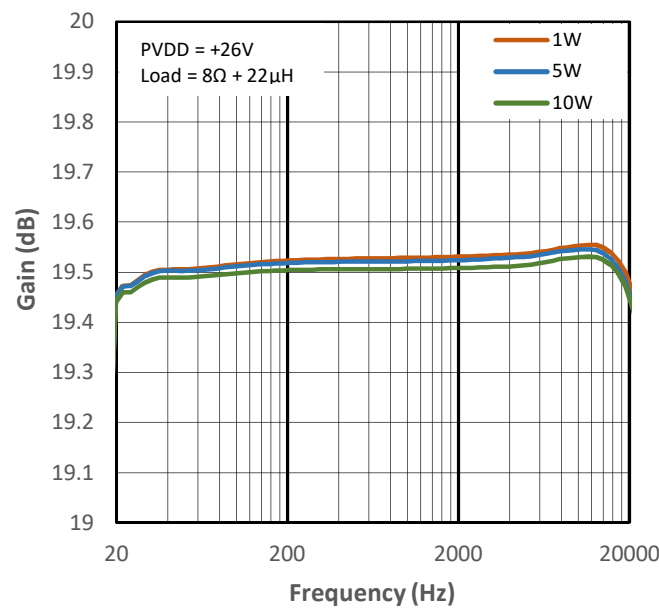
Figure 11-28 Low Gain vs Frequency for PMP4
