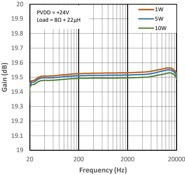
Figure 13-22 Low Gain vs Frequency for PMP1
