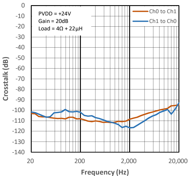
Figure 12-31 Crosstalk vs Frequency for PMP2
