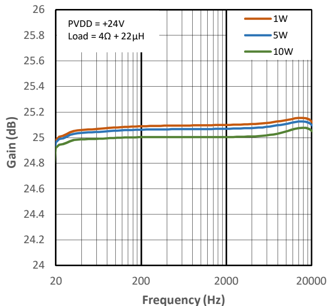
Figure 12-27 High Gain vs Frequency for PMP2
