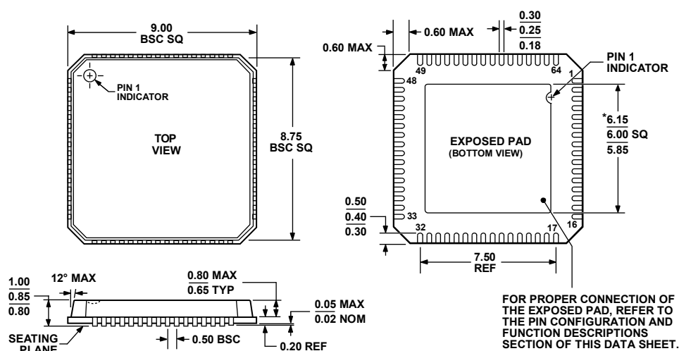
Figure 52. 64-Lead Lead Frame Chip Scale Package [LFCSP_VQ] 9 mm × 9 mm Body, Very Thin Quad (CP-64-2)
