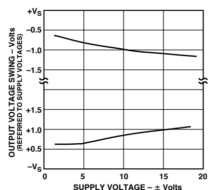
Figure 19. Output Voltage Swing vs. Supply Voltage
