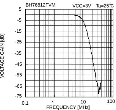
Fig. 22 Frequency characteristic
