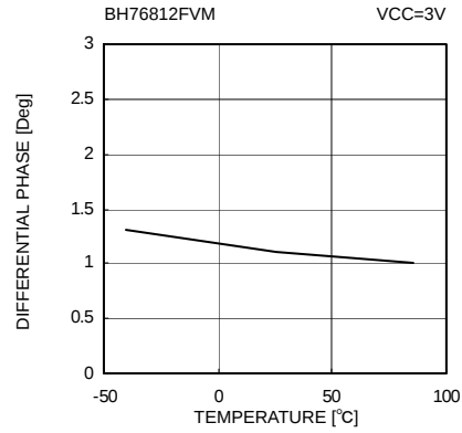
Fig. 39 Differential phase vs. Temperature
