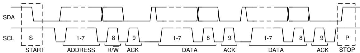
Figure 8-17. Complete Data Transfer on the I²C Bus
