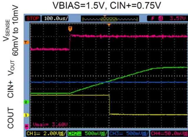
Current Limiter Falling Edge V_{BIAS} = 1.5V , C_{IN+} = 0.75V
