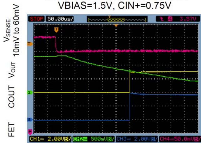
Circuit Breaker with Current Limiter V_{BIAS} = 1.5V , C_{IN+} = 0.75V
