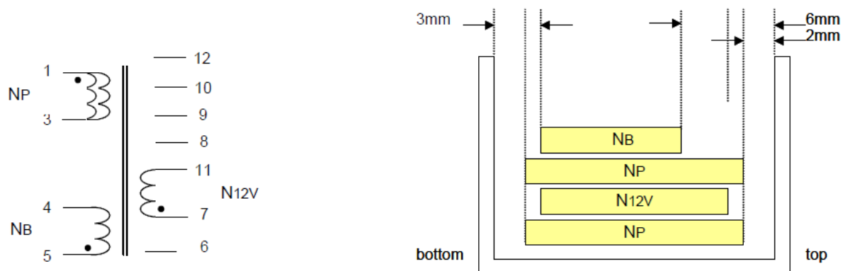
Figure 26. Transformer Specification
