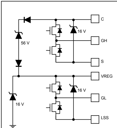
Figure 9a: Gate Drive Outputs
