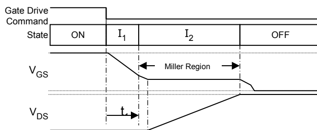
Figure 7c: On-to-Off Transition (Gate Drive)
