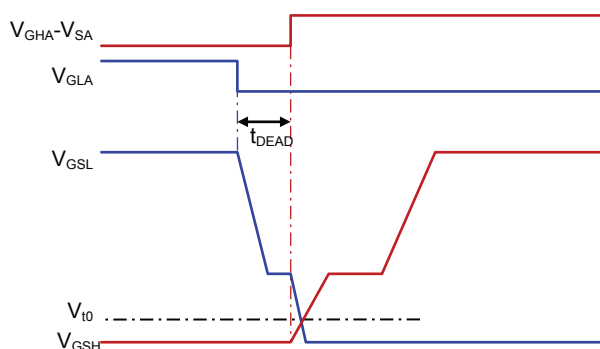
Figure 8: Minimum Dead Time
