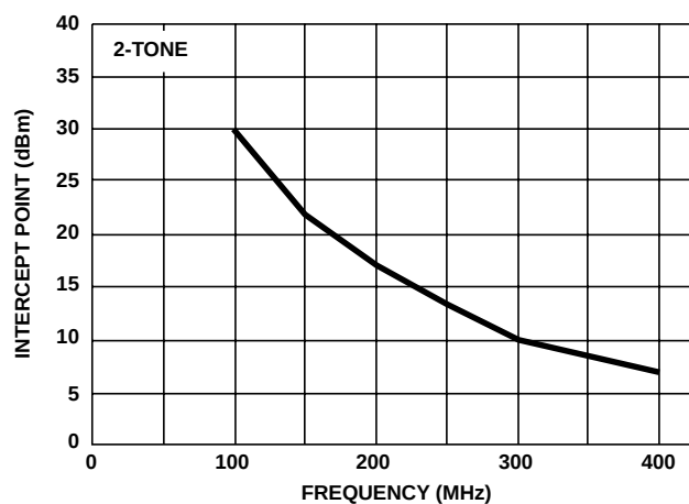
FIGURE 20. 3rd ORDER INTERMODULATION INTERCEPT
