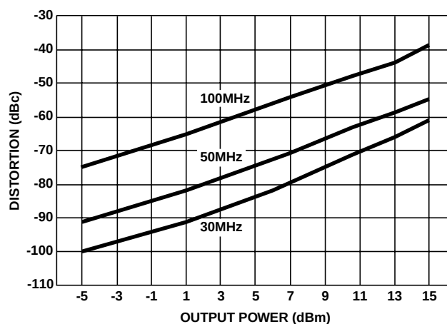
FIGURE 22. 3rd HARMONIC DISTORTION vs P_{\text{OUT}}
