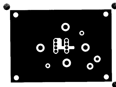
BOTTOM LAYOUT
