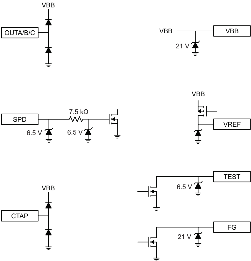
Figure 11: Pin Diagrams
