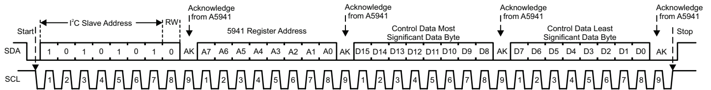
Figure 8: Write Command
