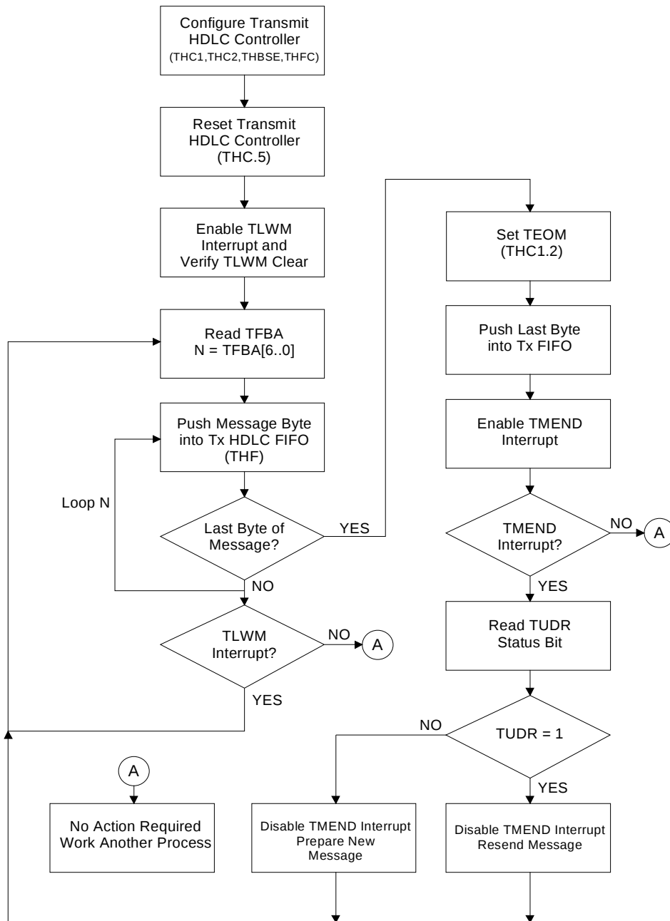
Figure 8-16. HDLC Message Transmit Example
