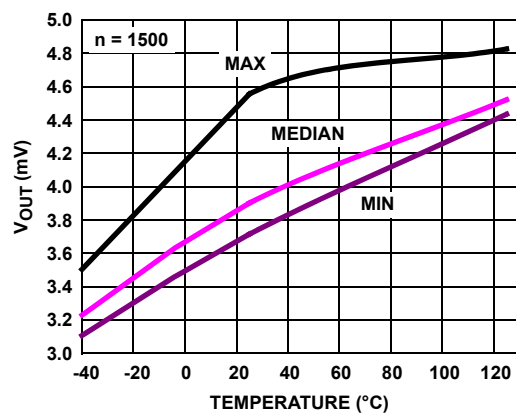
FIGURE 27. V_{OUT} LOW vs TEMPERATURE, V_S = \pm 2.5V , R_L = 100k
