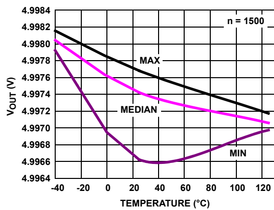
FIGURE 25. V_{OUT} HIGH vs TEMPERATURE, V_S = \pm 2.5V , R_L = 100k
