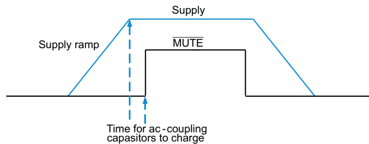
Figure 10. Power-Up and Power-Down Sequence
