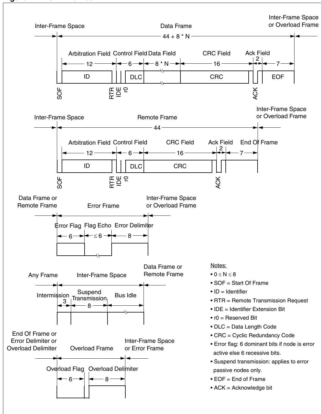
Figure 41. CAN frames
