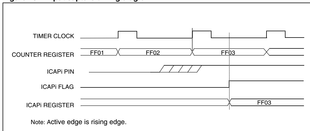
Figure 25. Input capture timing diagram
