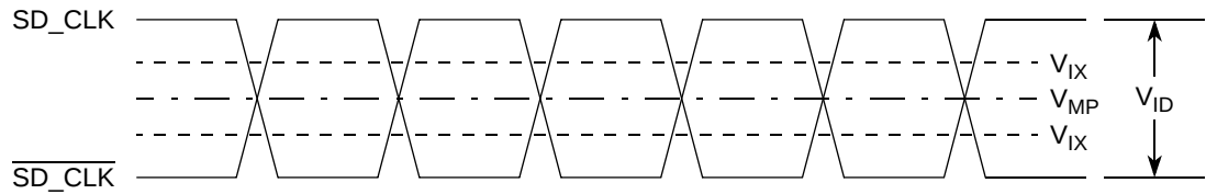
Figure 15. SD_CLK and SD_CLK Crossover Timing
