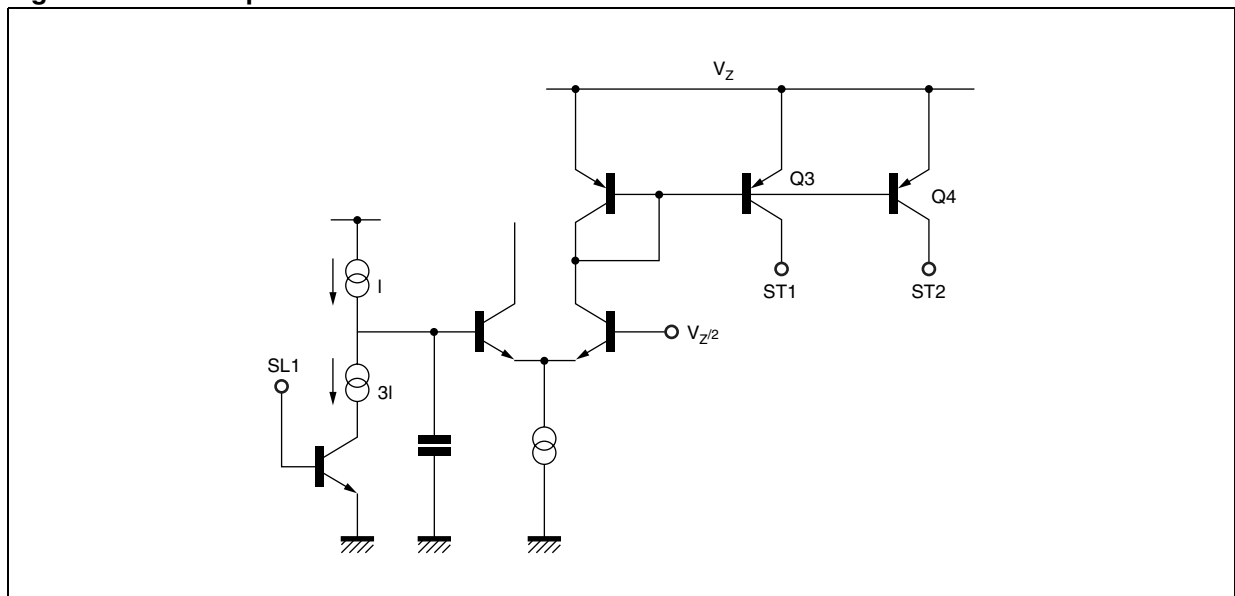
Figure 5. Frame Separator
