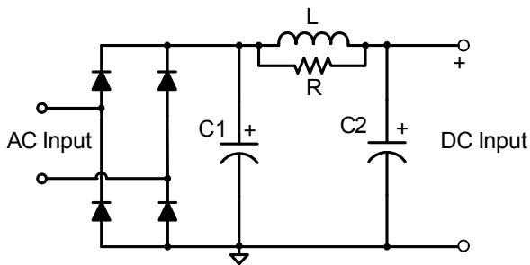
Figure 9: Input Filter
