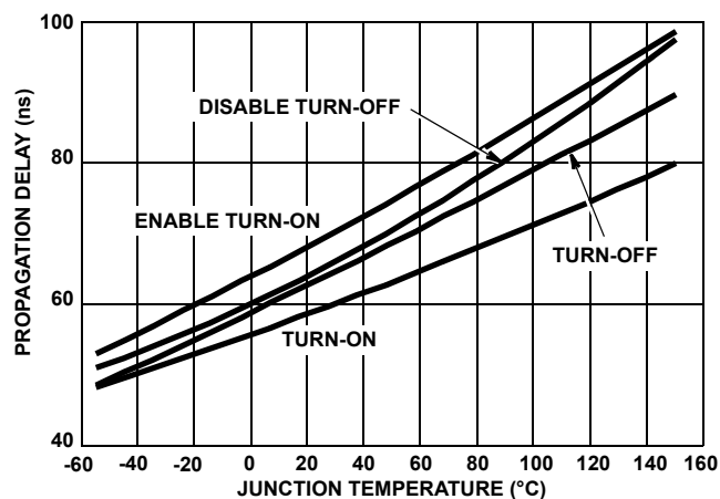
FIGURE 8. PROPAGATION DELAY
