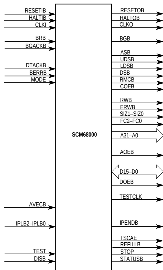
Figure 2-1. Input/Output Signals
