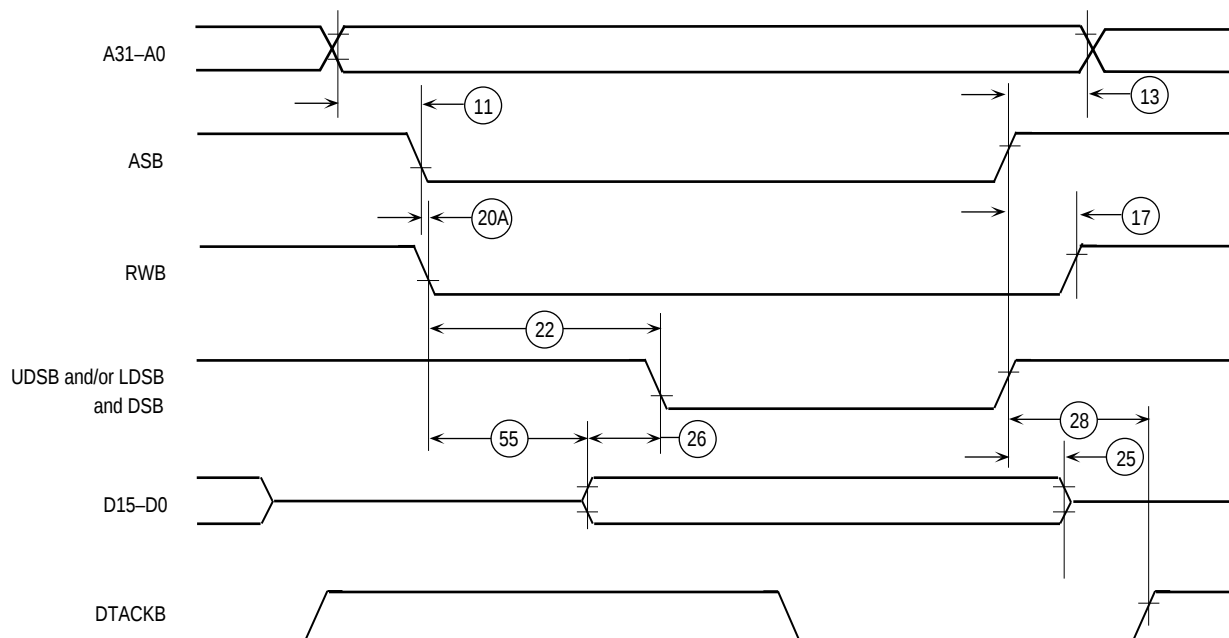
Figure 3-32. Pseudo-Asynchronous Write Cycle
