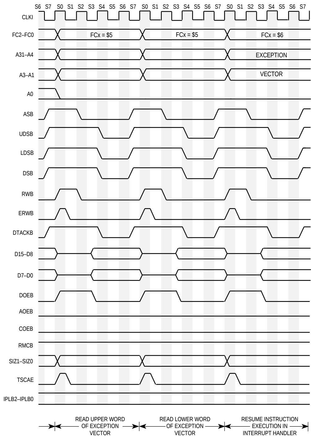
Figure 4-2. Interrupt Acknowledge Cycle Timing Diagram (Sheet 3 of 3)
