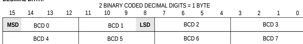
Figure 1-6. Data Organization in Memory
