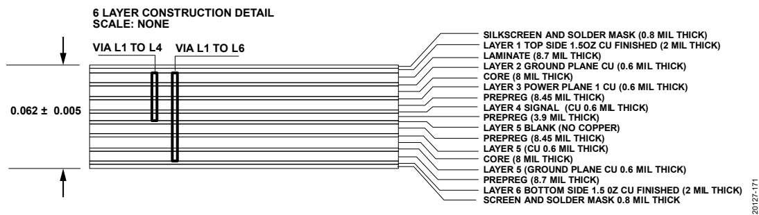
Figure 71. PCB Stackup
