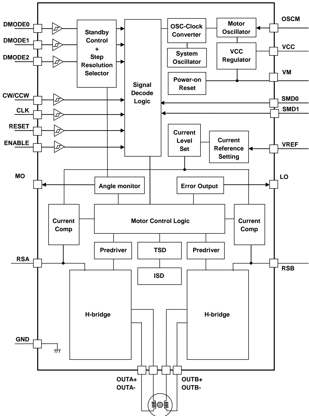
TB67S209 Block diagram
