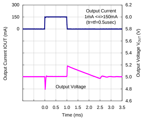
VR=5.0V, C OUT =10μF
