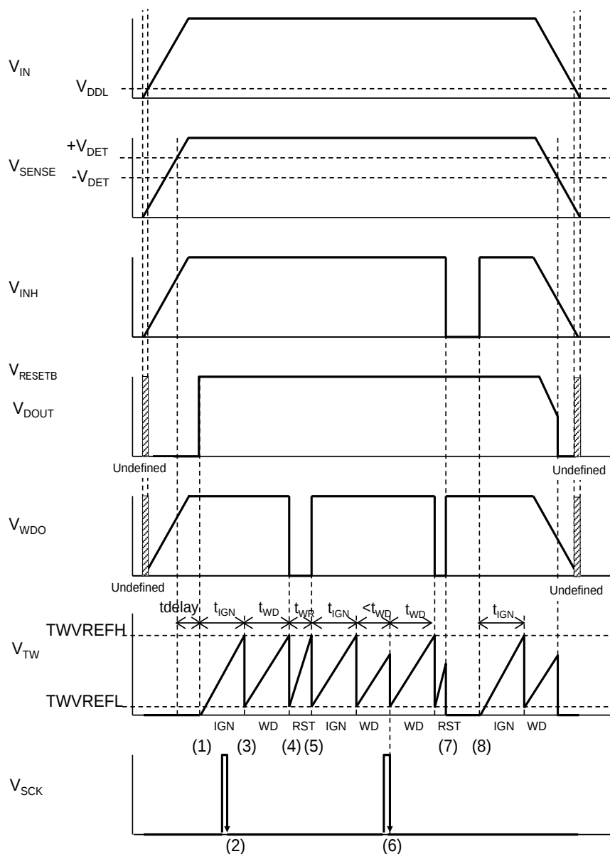
R5111xxx2C WDT Timing Chart
