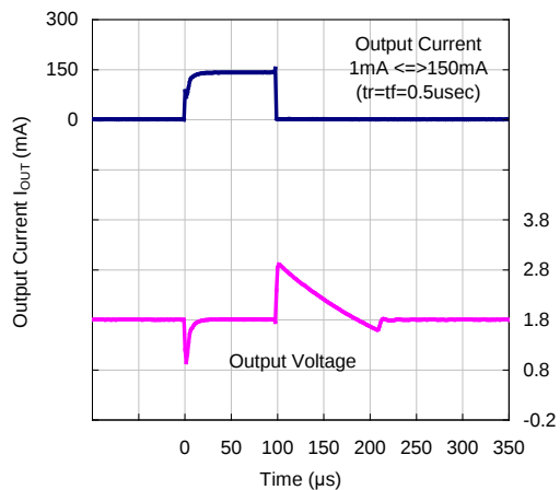
VR=1.8V, C OUT =0.1μF
