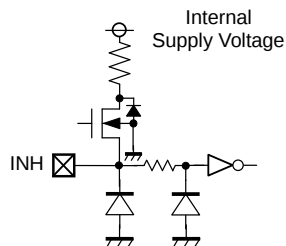
<INH Pin ( R5111xxx2x) >
