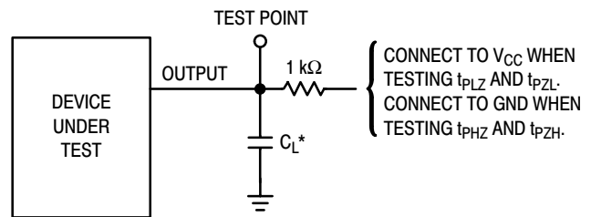
Figure 8. Test Circuit
