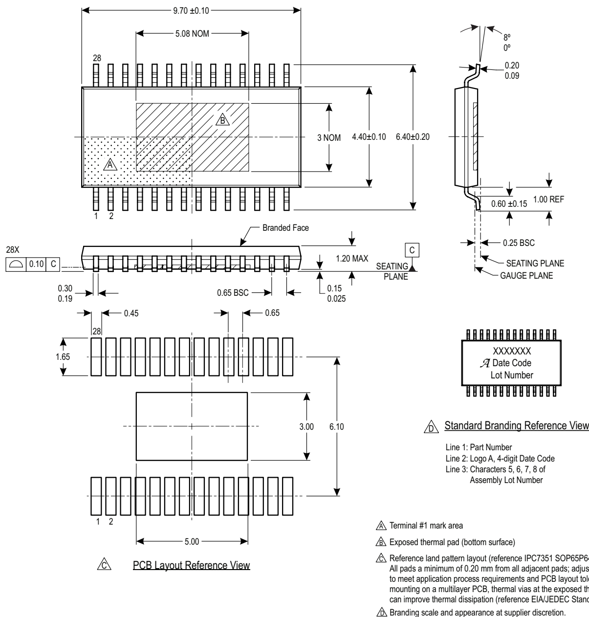
Figure 8: LP Package, 28-pin TSSOP with Exposed Thermal Pad
