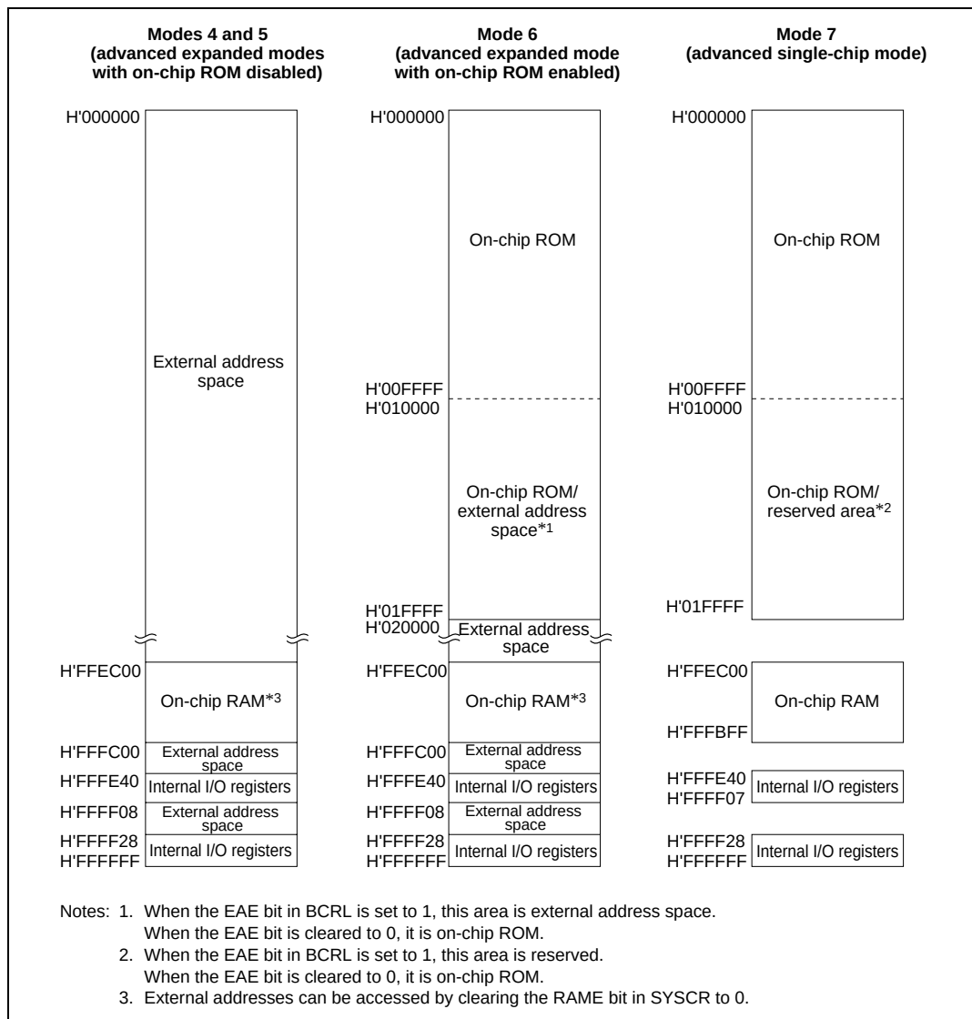
Figure 3.1 Memory Map in Each Operating Mode in the H8S/2345 (cont)
