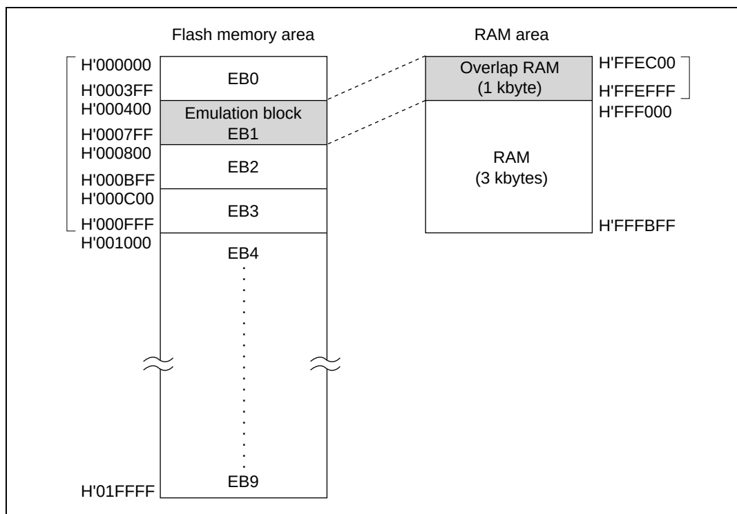
Figure 17.14 Example of Overlap Between Flash Memory Area and RAM Area (When RAMS = 1, RAM1 = 0, and RAM0 = 1)
