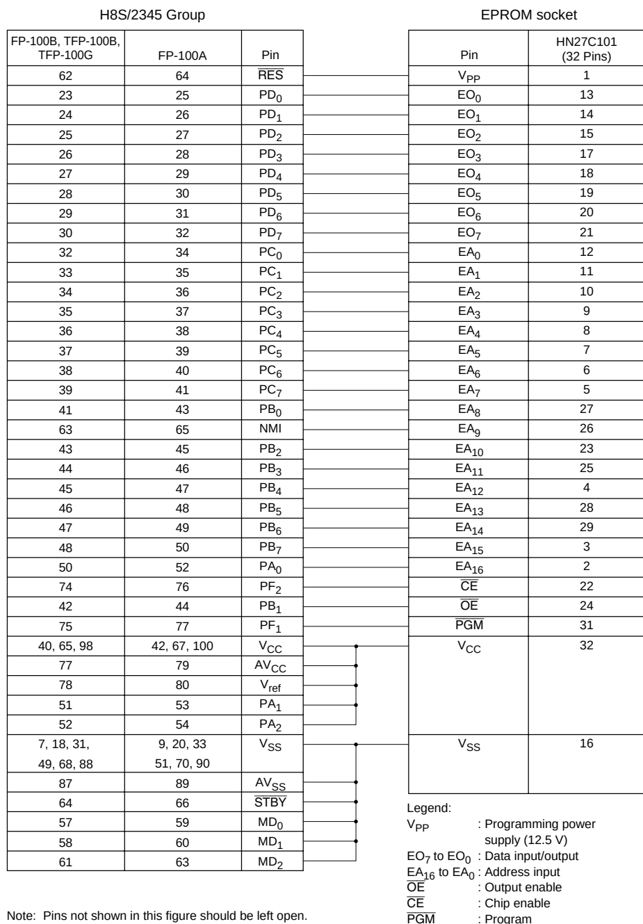
Figure 17.2 Wiring of 100-Pin/32-Pin Socket Adapter
