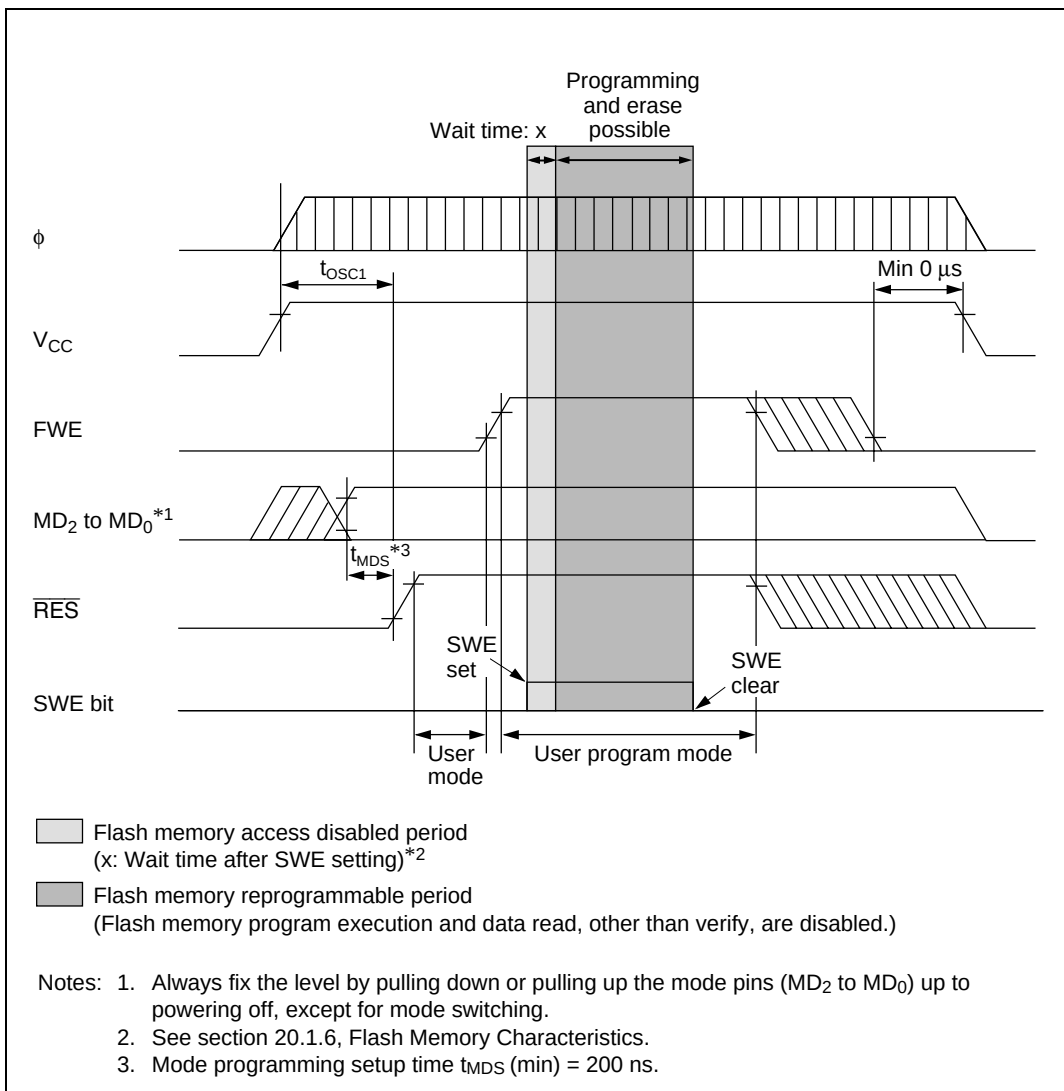
Figure 17.37 Powering On/Off Timing (User Program Mode)
