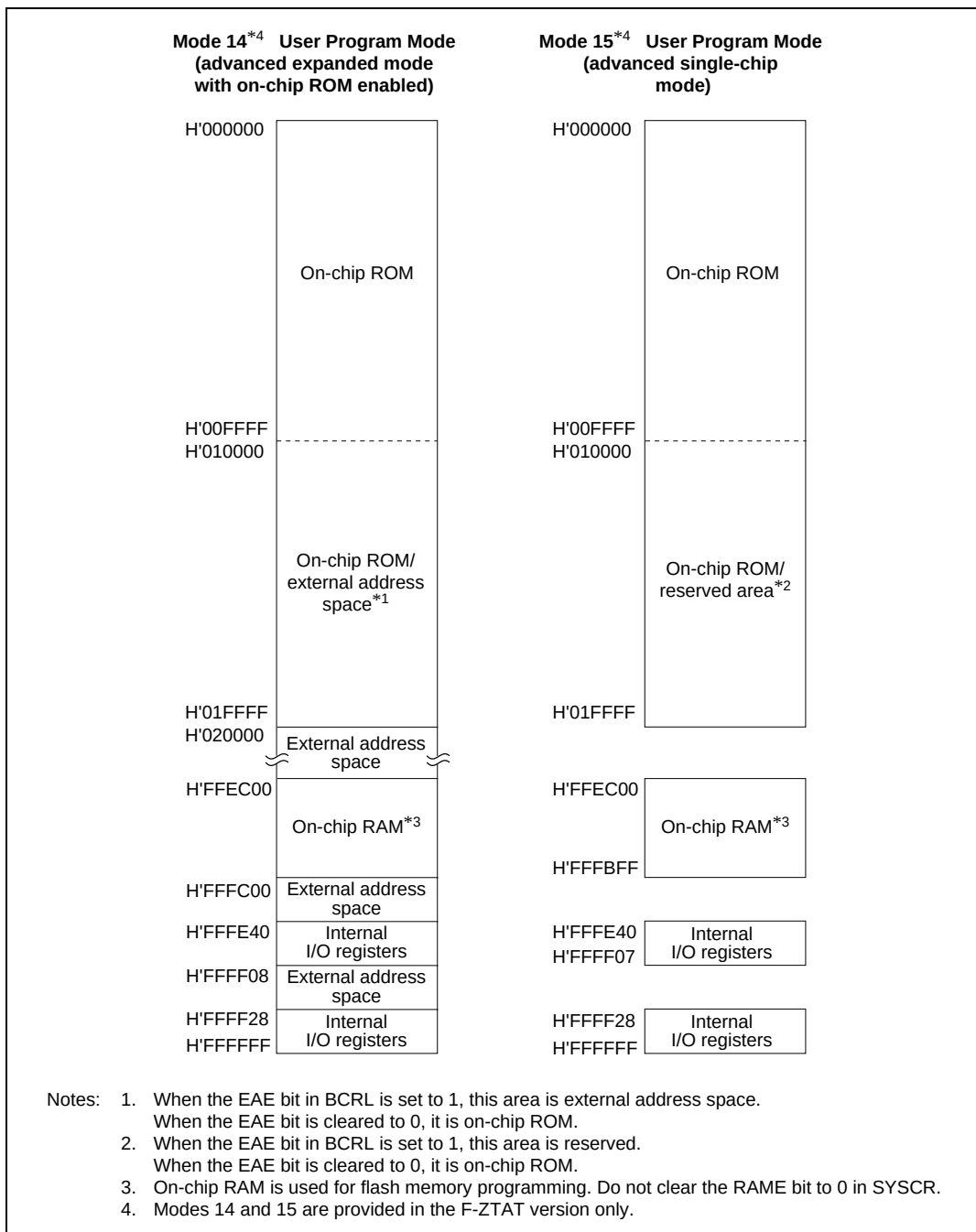
Figure 3.1 Memory Map in Each Operating Mode in the H8S/2345 (cont)
