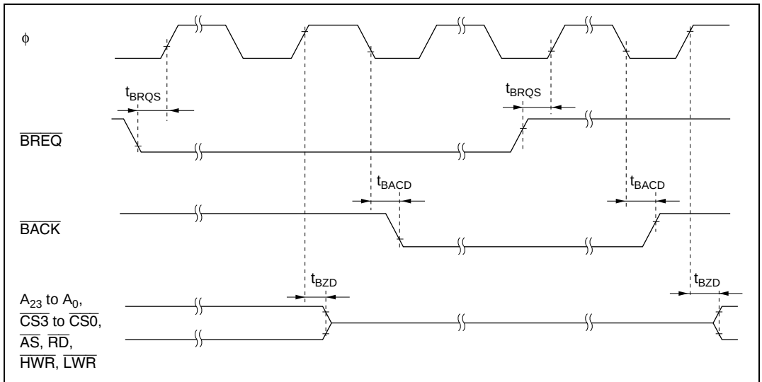
Figure 20.16 External Bus Release Timing
