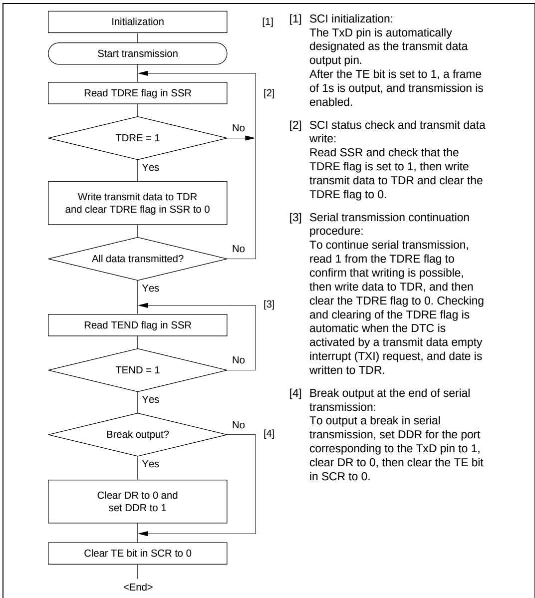
Figure 12.5 Sample Serial Transmission Flowchart
