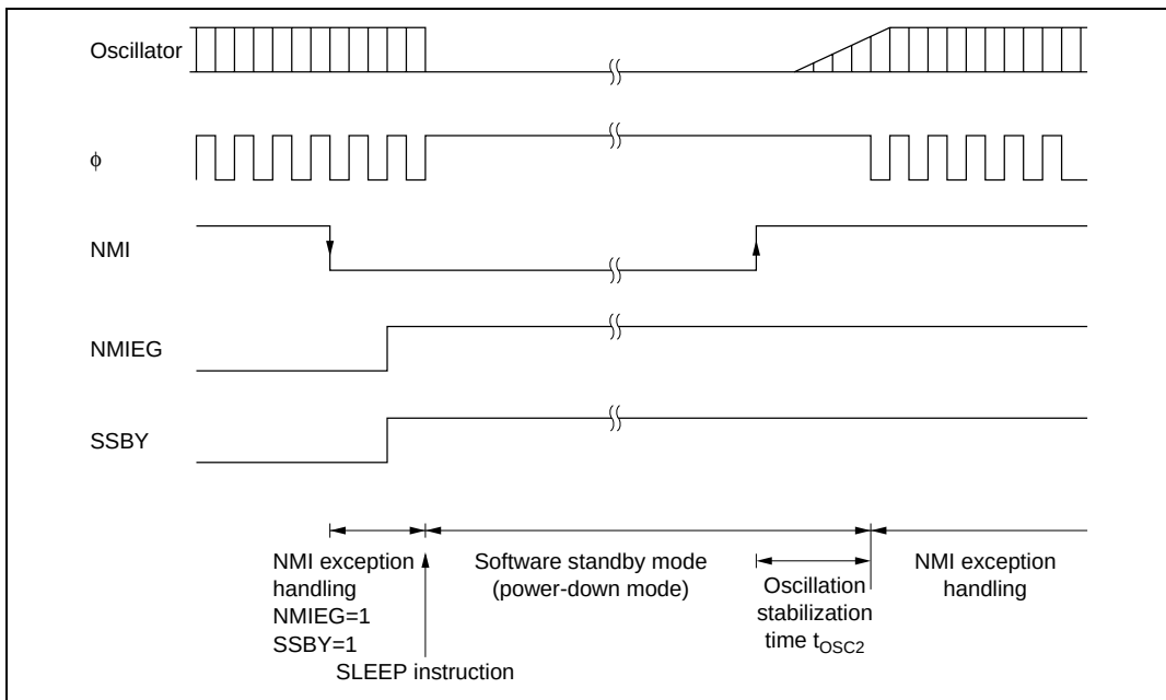
Figure 19.2 Software Standby Mode Application Example
