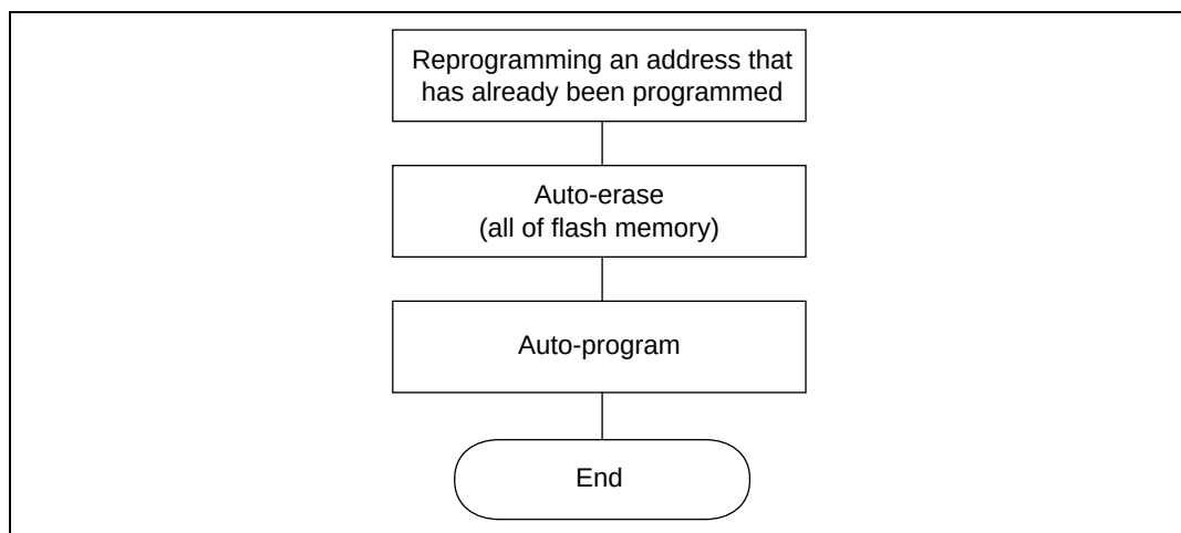
Figure 17.35 Reprogramming an Address that has Already Been Programmed
