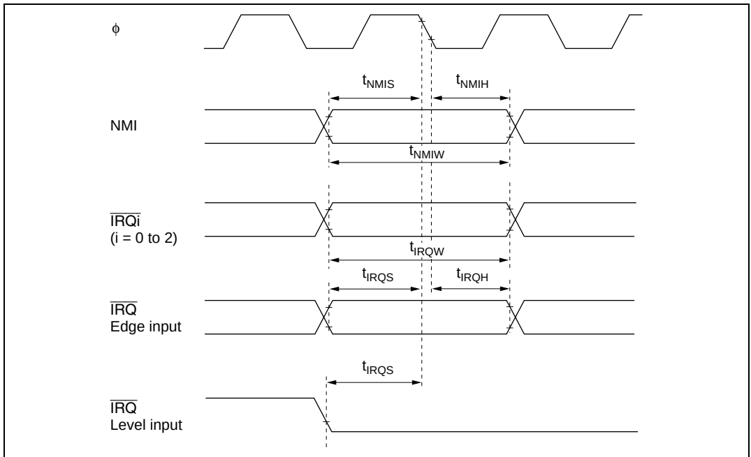
Figure 20.10 Interrupt Input Timing
