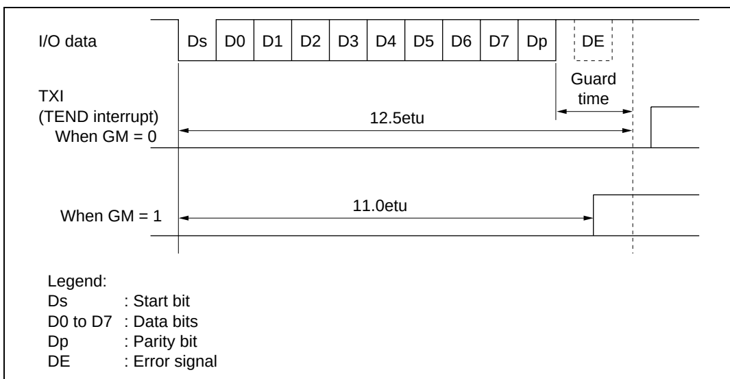
Figure 13.6 TEND Flag Generation Timing in Transmission Operation
