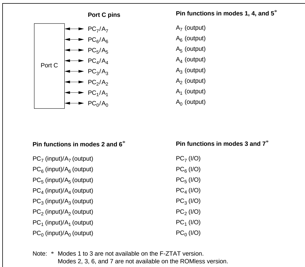
Figure 8.13 Port C Pin Functions
