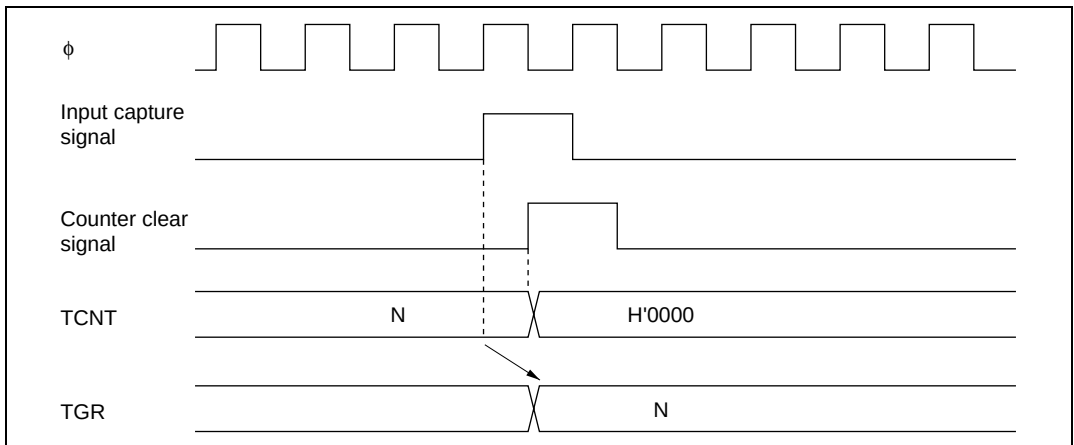
Figure 9.39 Counter Clear Timing (Input Capture)
