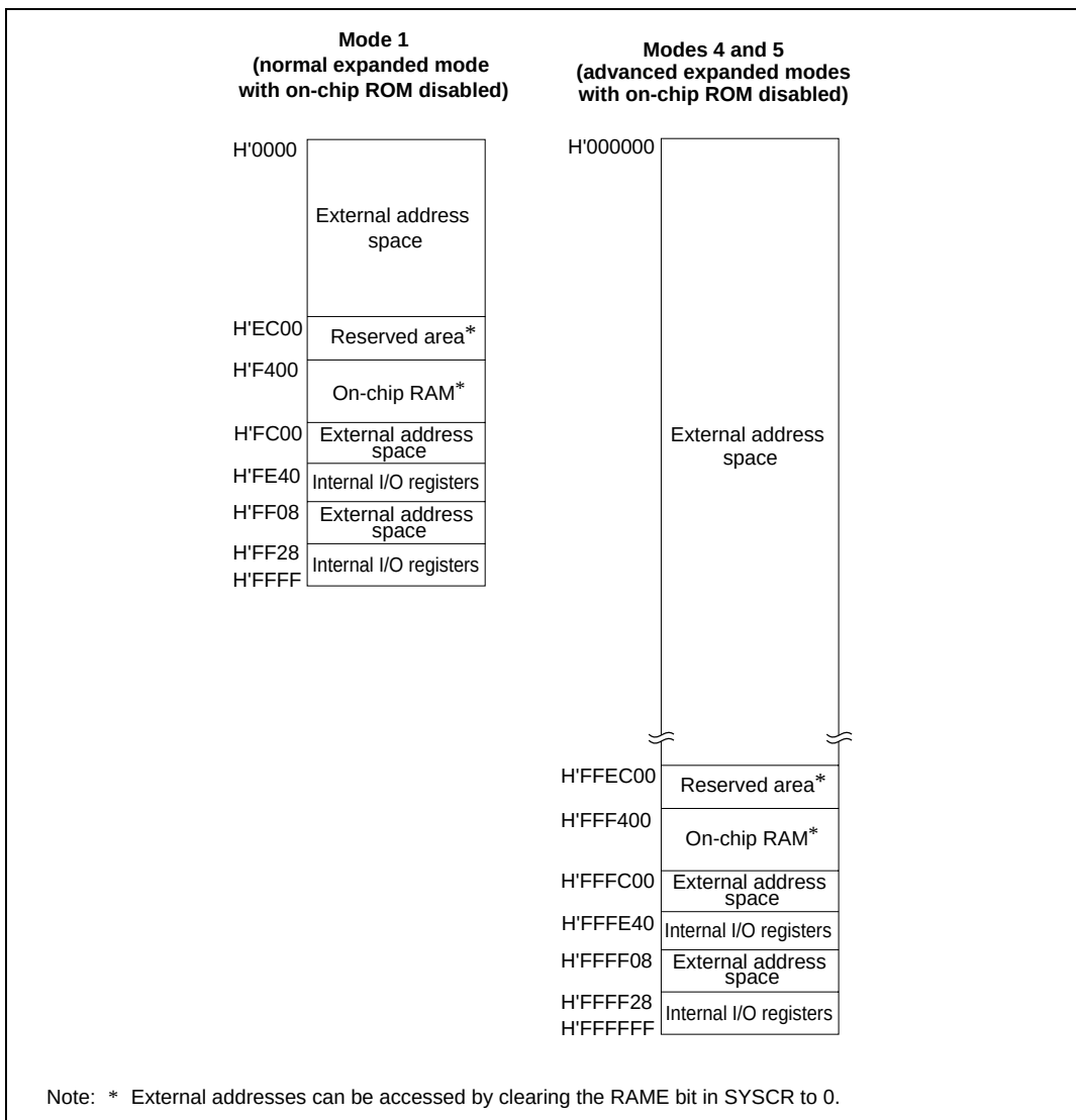
Figure 3.5 Memory Map in Each Operating Mode in the H8S/2340 (Modes 1, 4, and 5 Only)
