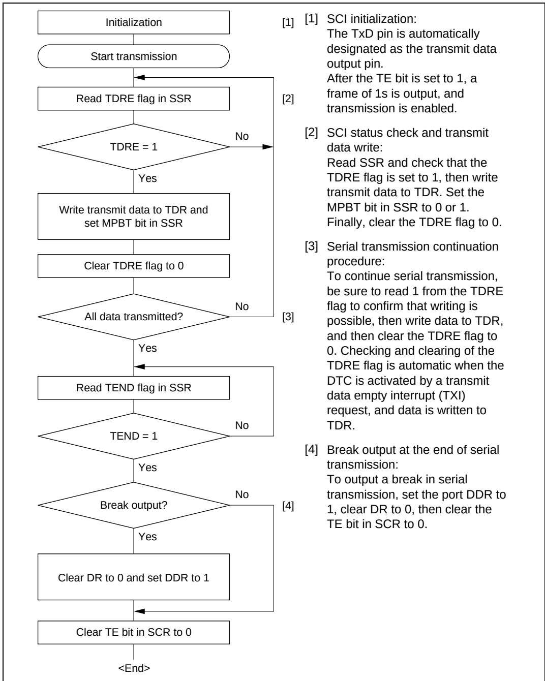
Figure 12.10 Sample Multiprocessor Serial Transmission Flowchart
