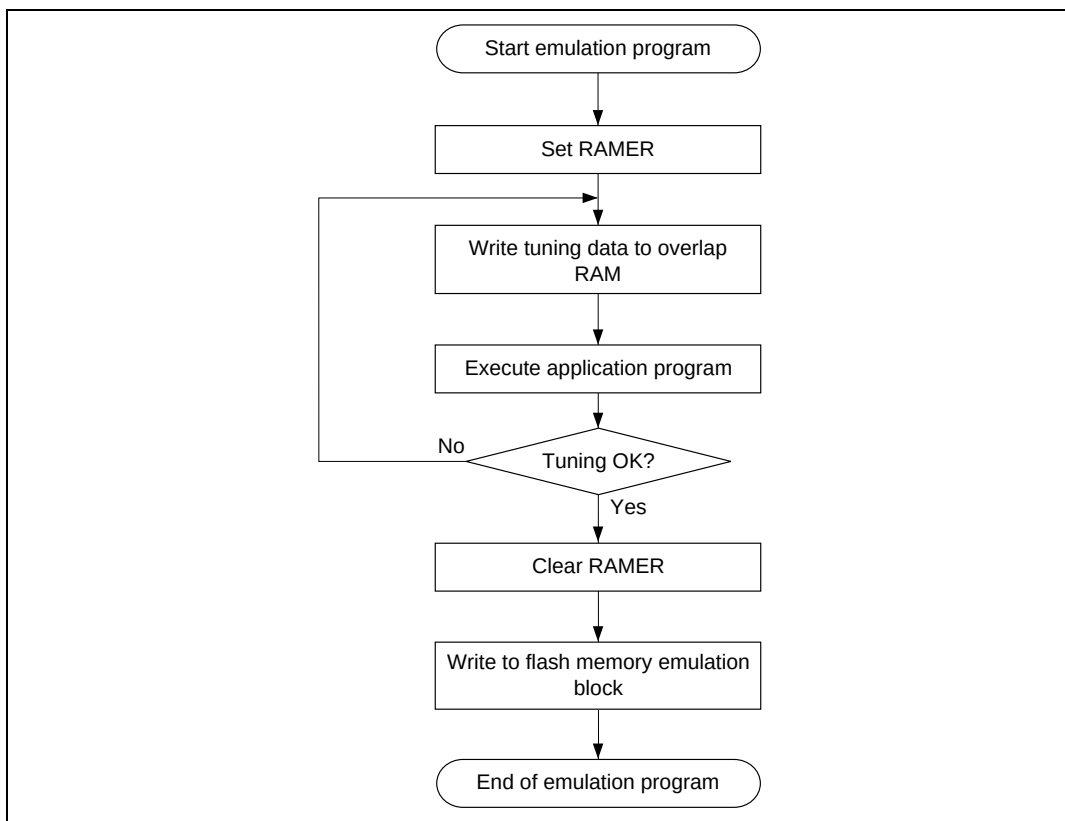
Figure 17.24 Flowchart for Flash Memory Emulation in RAM
