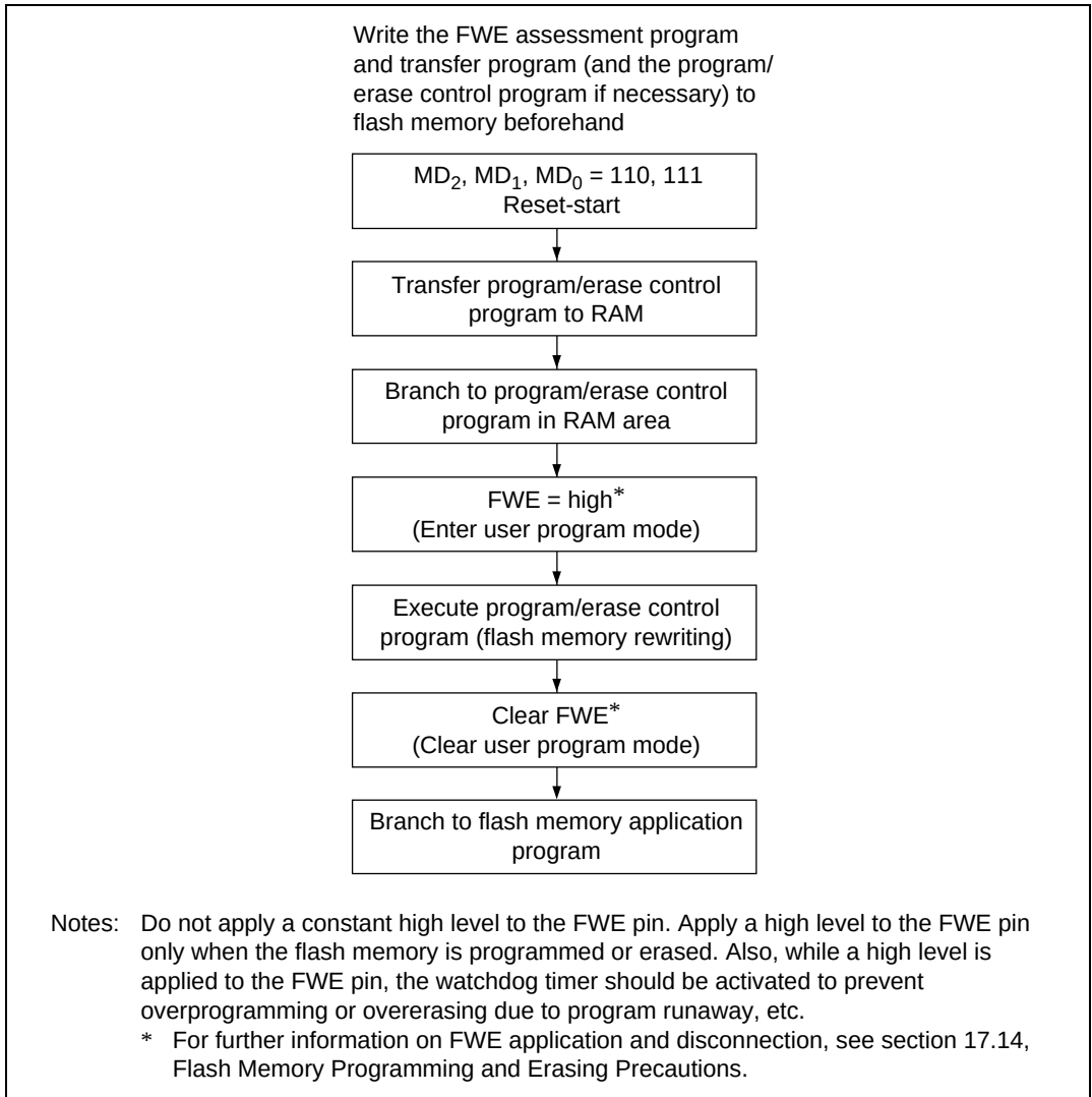
Figure 17.19 User Program Mode Execution Procedure
