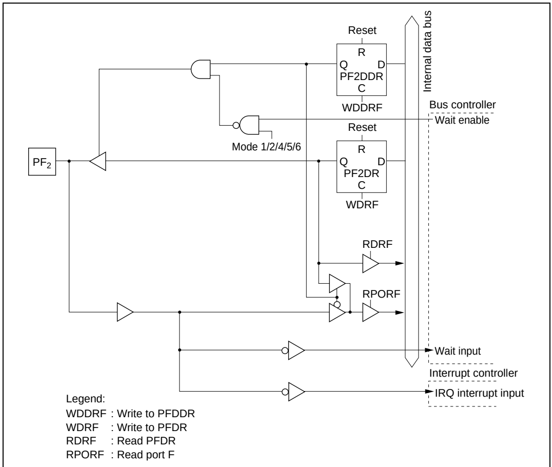
Figure C.10 (c) Port F Block Diagram (Pin PF 2 )
