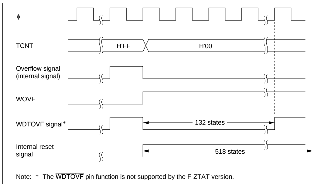
Figure 11.7 Timing of Setting of WO VF
