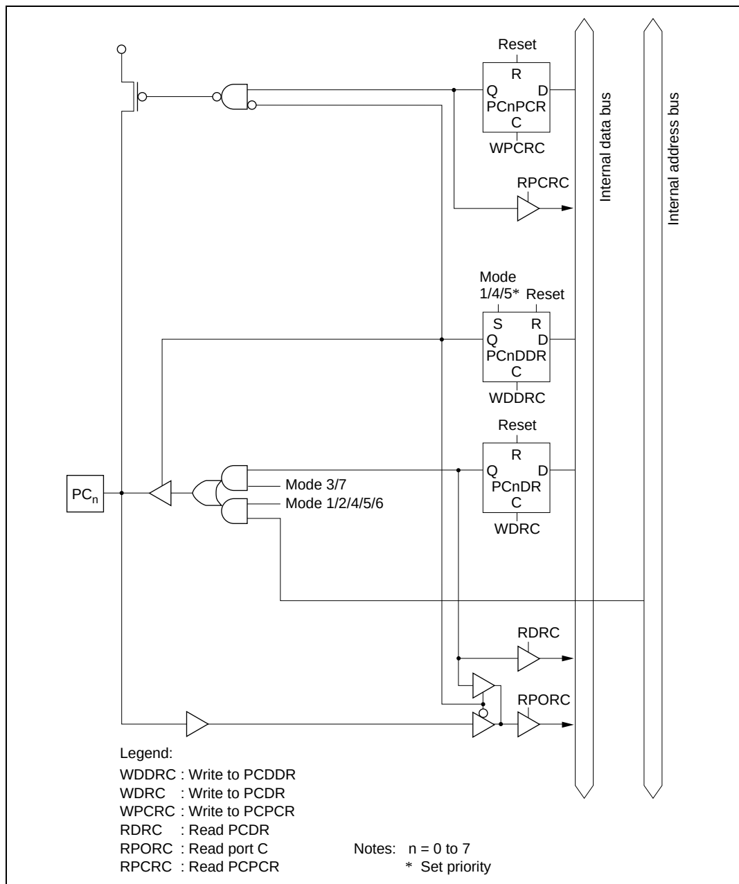
Figure C.7 Port C Block Diagram (Pin PC_n )
