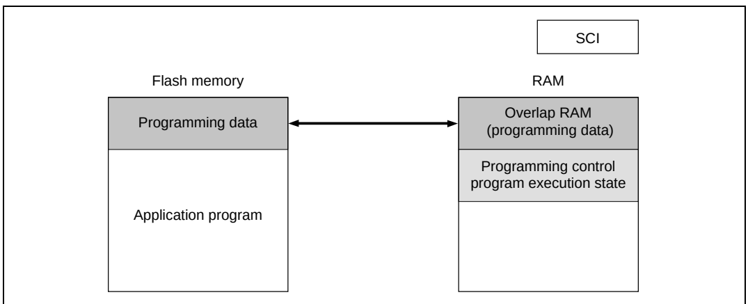
Figure 17.12 Writing Overlap Data in User Program Mode
