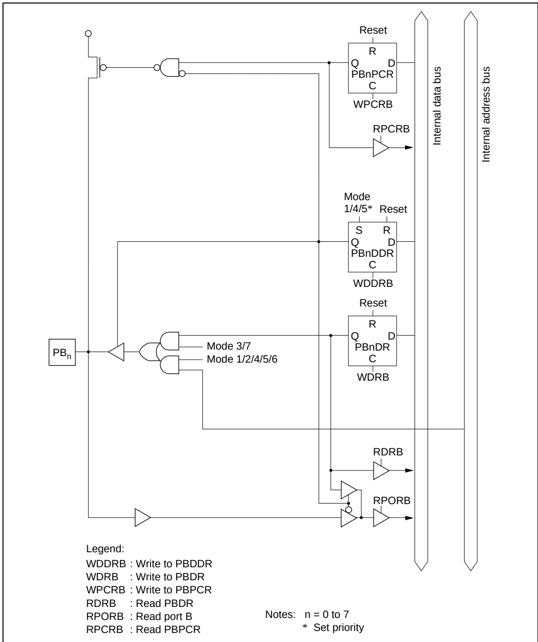
Figure C.6 Port B Block Diagram (Pin PB_n )
