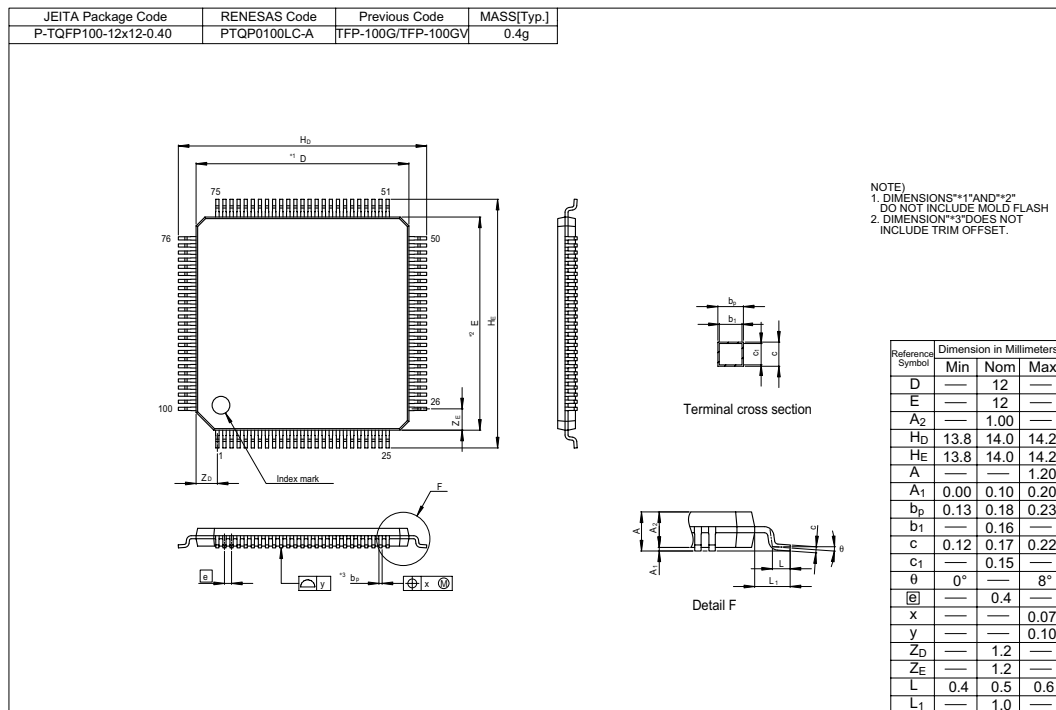
Figure G.2 TFP-100G Package Dimensions
