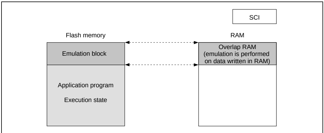
Figure 17.11 Reading Overlap Data in User Mode and User Program Mode
