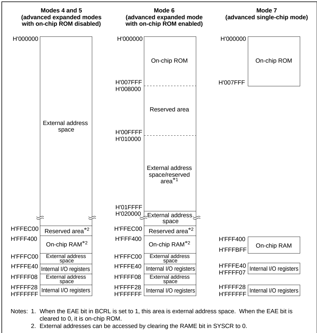
Figure 3.4 Memory Map in Each Operating Mode in the H8S/2341 (cont)
