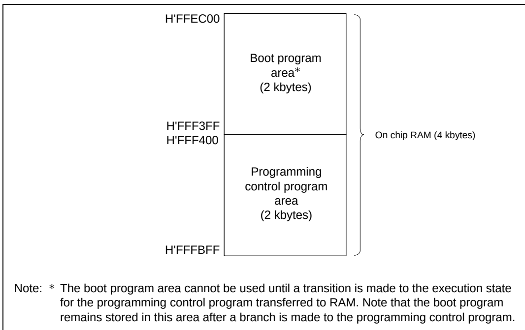
Figure 17.18 RAM Areas in Boot Mode
