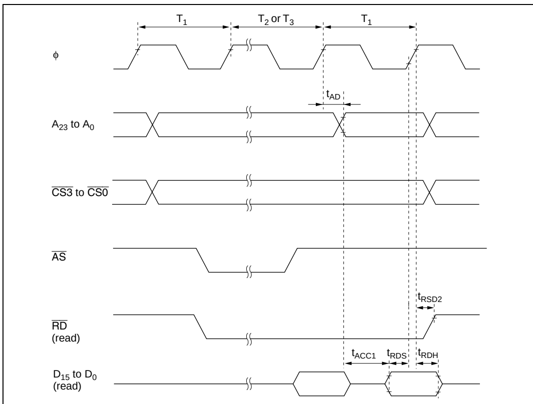
Figure 20.15 Burst ROM Access Timing (One-State Access)
