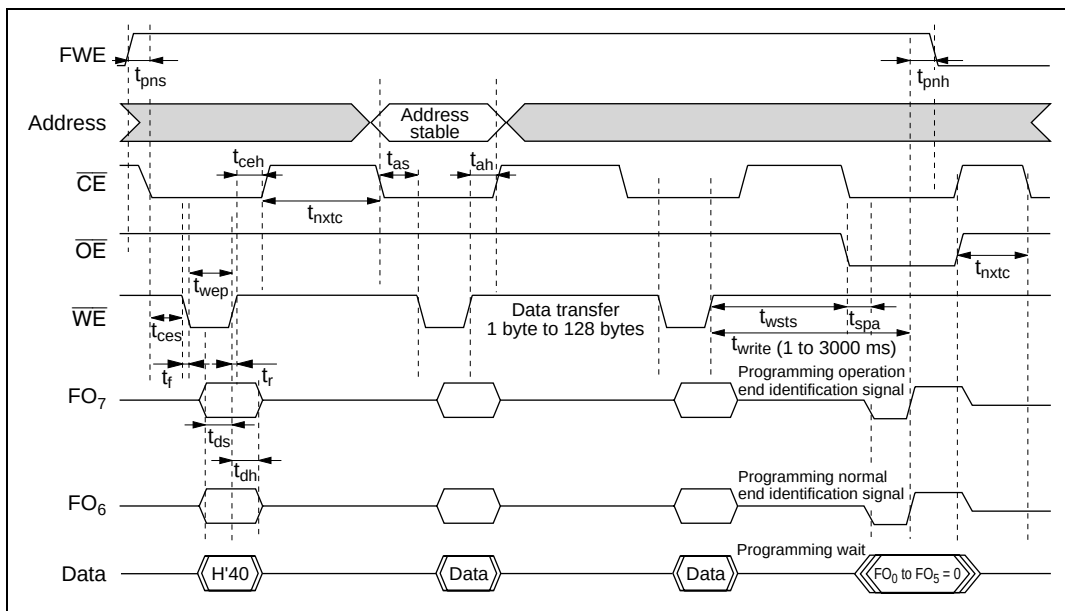
Figure 17.31 Auto-Program Mode Timing Waveforms
