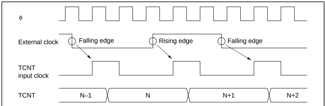
Figure 9.35 Count Timing in External Clock Operation
