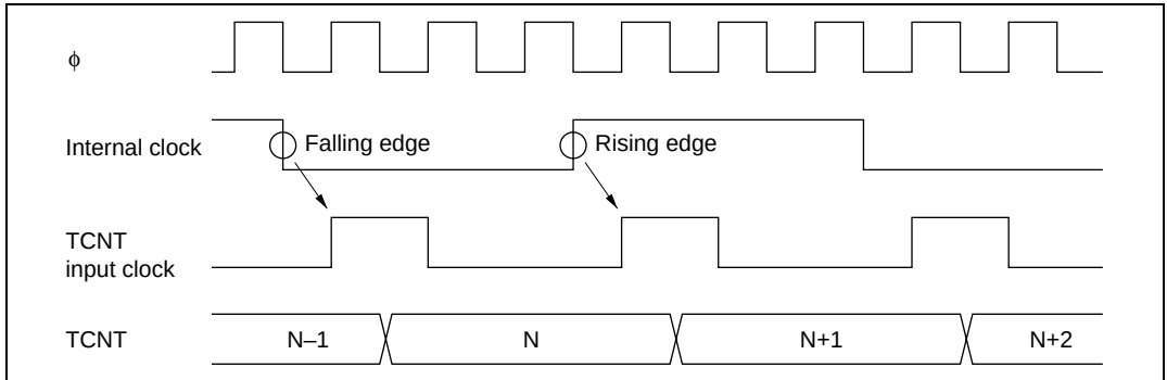
Figure 9.34 Count Timing in Internal Clock Operation
