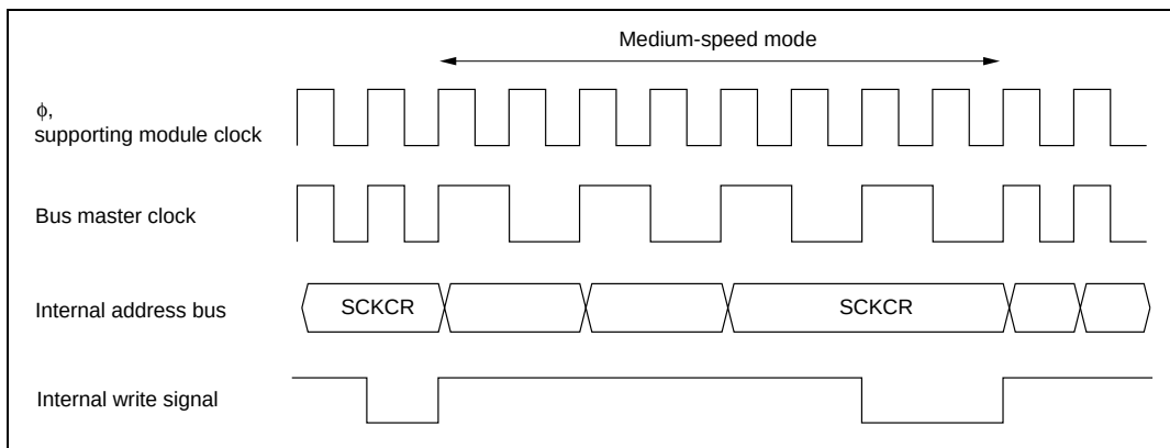
Figure 19.1 Medium-Speed Mode Transition and Clearance Timing
