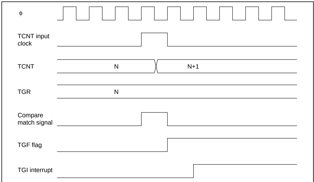
Figure 9.42 TGI Interrupt Timing (Compare Match)
