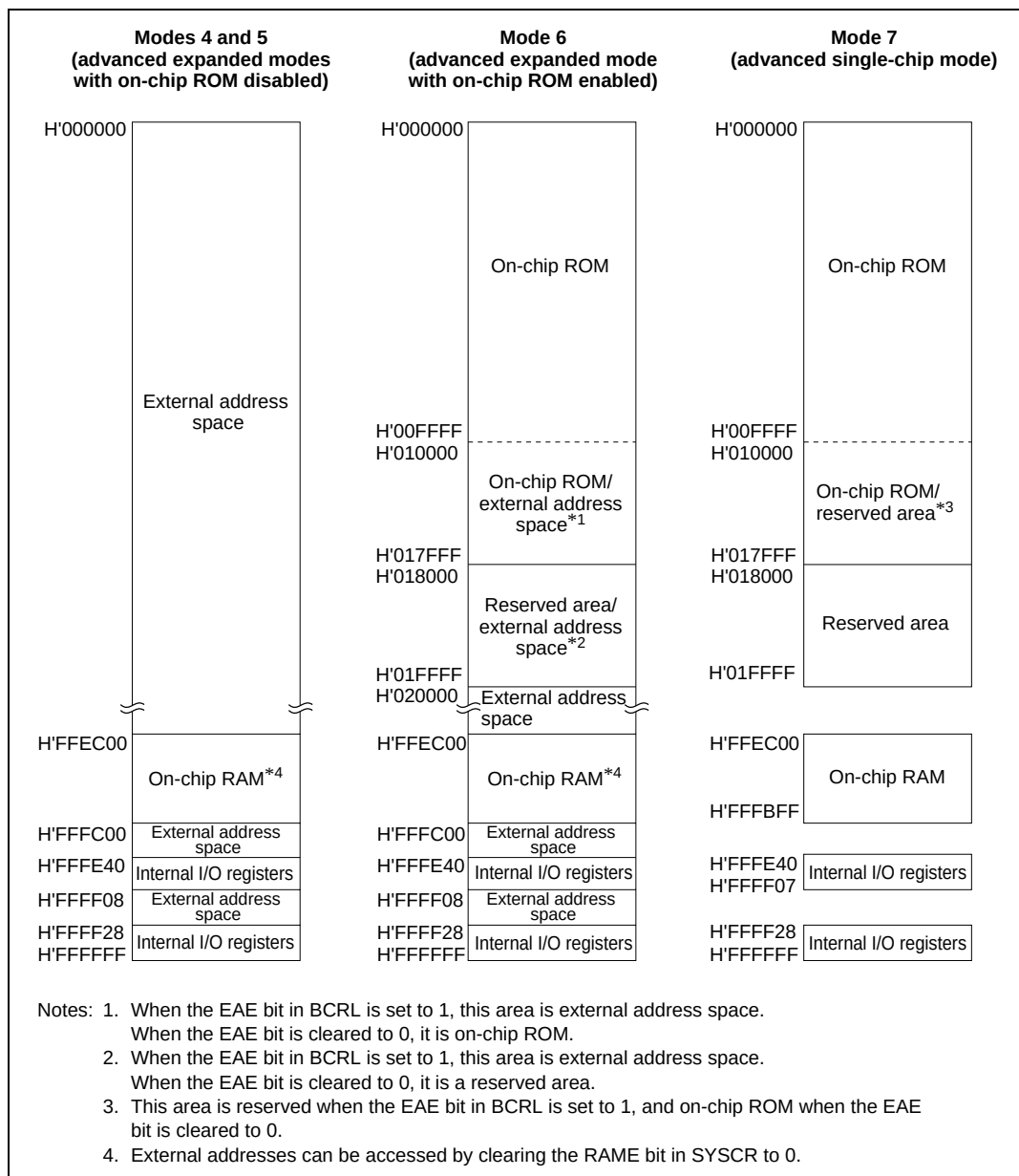
Figure 3.2 Memory Map in Each Operating Mode in the H8S/2344 (cont)
