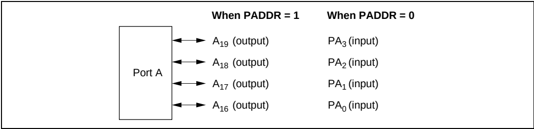
Figure 8.8 Port A Pin Functions (Mode 6)*
