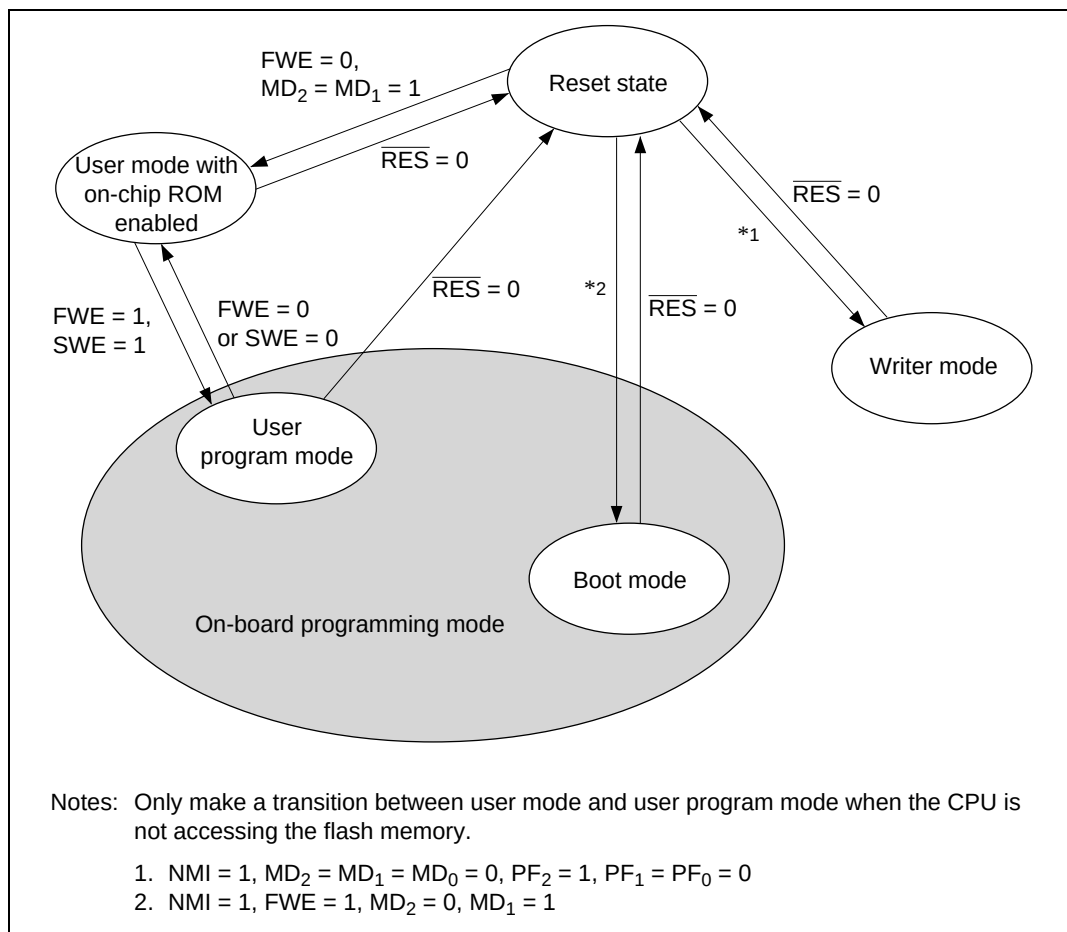
Figure 17.8 Flash Memory Mode Transitions
