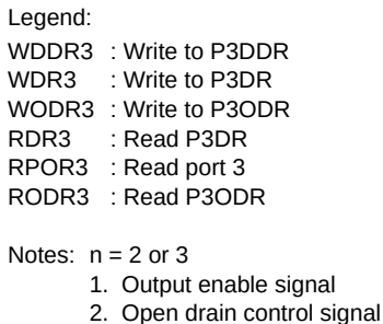
Figure C.3 (b) Port 3 Block Diagram (Pins P3 2 and P3 3 )
