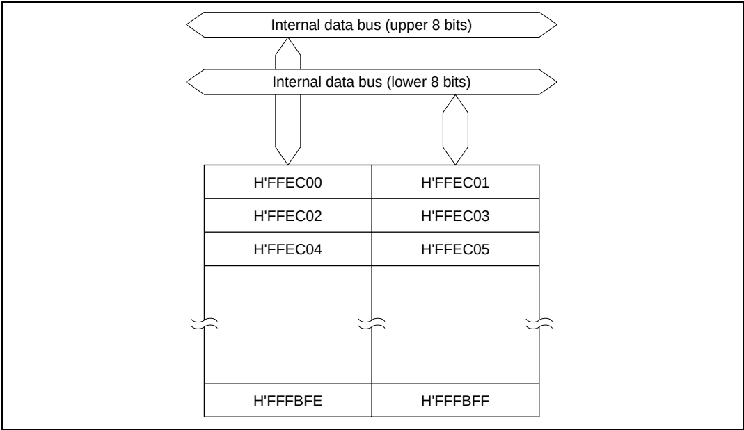
Figure 16.1 Block Diagram of RAM (H8S/2345, Advanced Mode)
