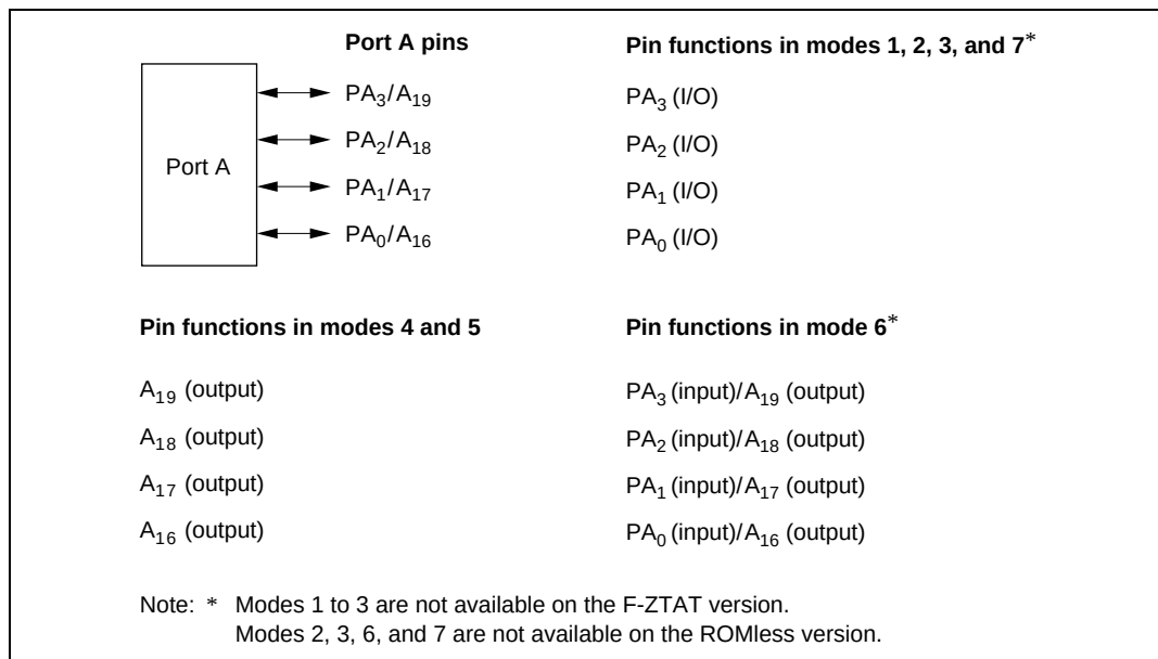
Figure 8.5 Port A Pin Functions
