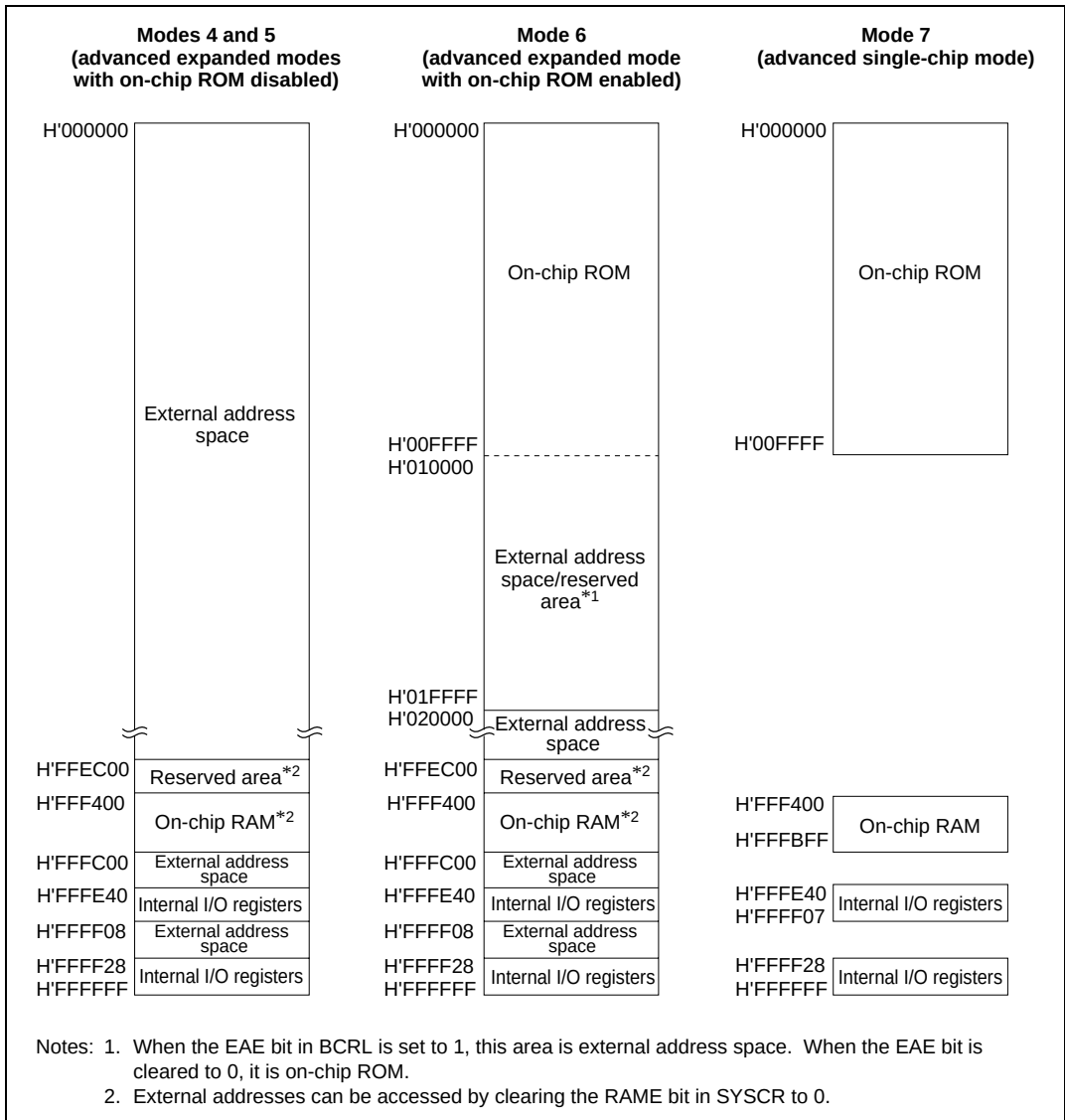
Figure 3.3 Memory Map in Each Operating Mode in the H8S/2343 (cont)
