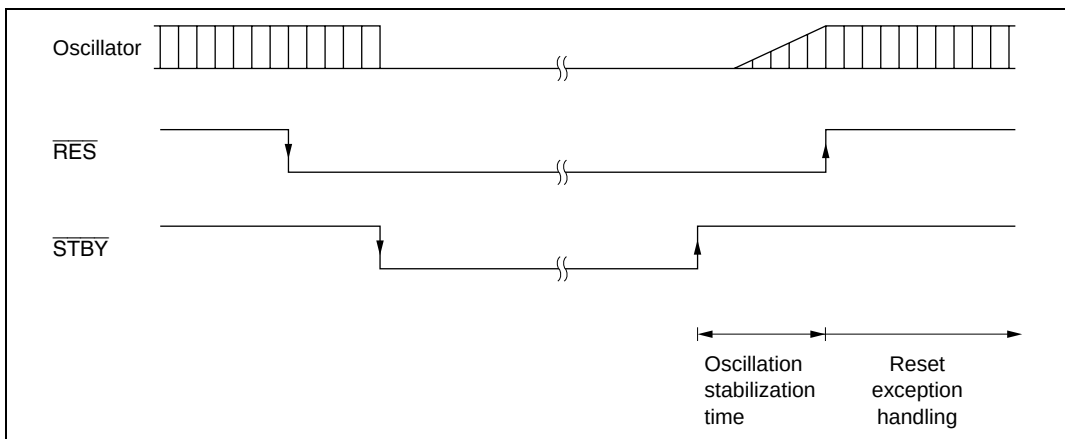
Figure 19.3 Hardware Standby Mode Timing (Example)
