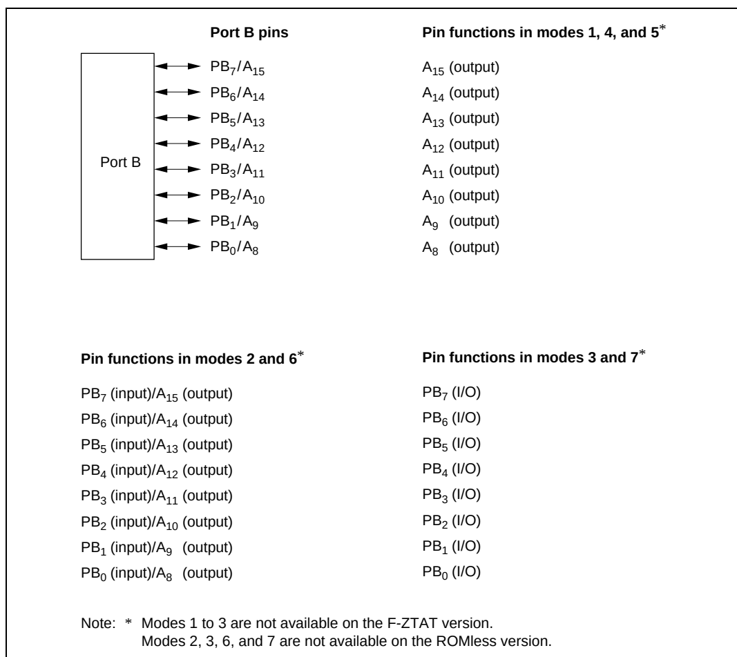
Figure 8.9 Port B Pin Functions
