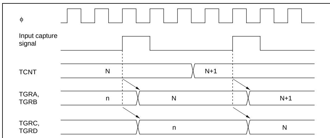
Figure 9.41 Buffer Operation Timing (Input Capture)
