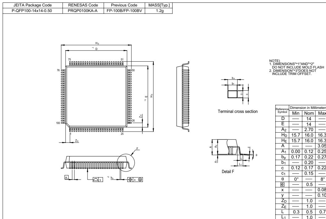
Figure G.4 FP-100B Package Dimensions
