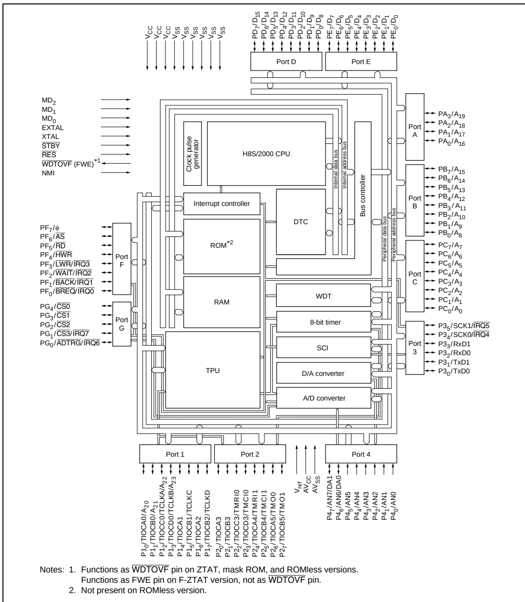
Figure 1.1 Block Diagram
