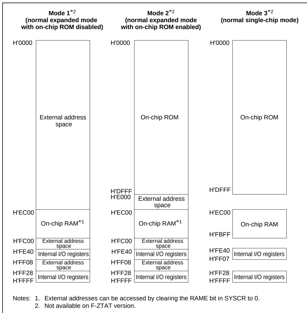
Figure 3.1 Memory Map in Each Operating Mode in the H8S/2345
