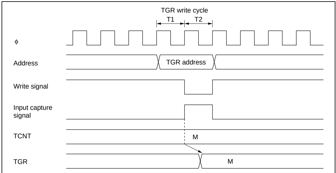
Figure 9.54 Contention between TGR Write and Input Capture
