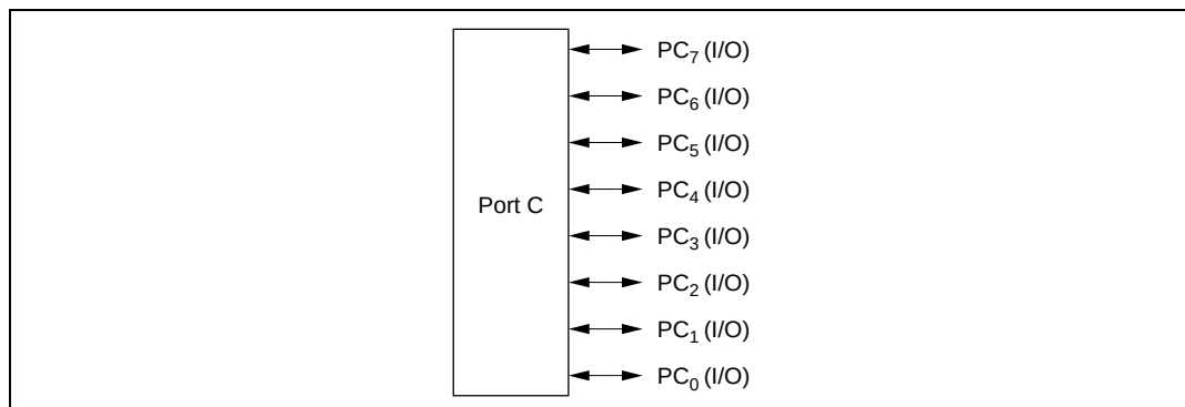
Figure 8.16 Port C Pin Functions (Modes 3 and 7)*
