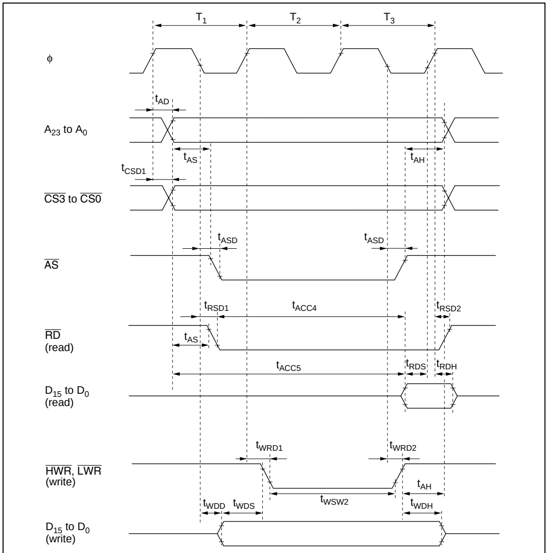
Figure 20.12 Basic Bus Timing (Three-State Access)
