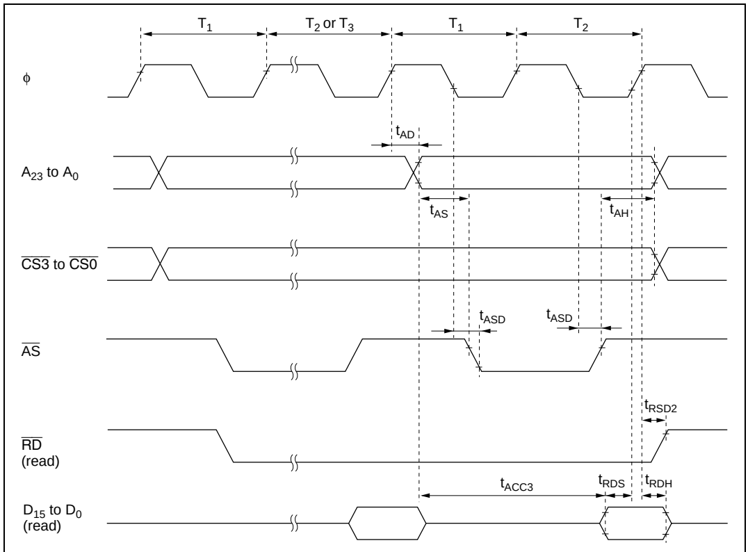
Figure 20.14 Burst ROM Access Timing (Two-State Access)
