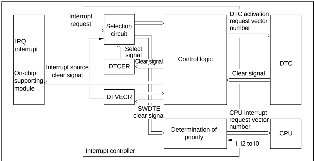
Figure 5.9 Interrupt Control for DTC and DMAC
