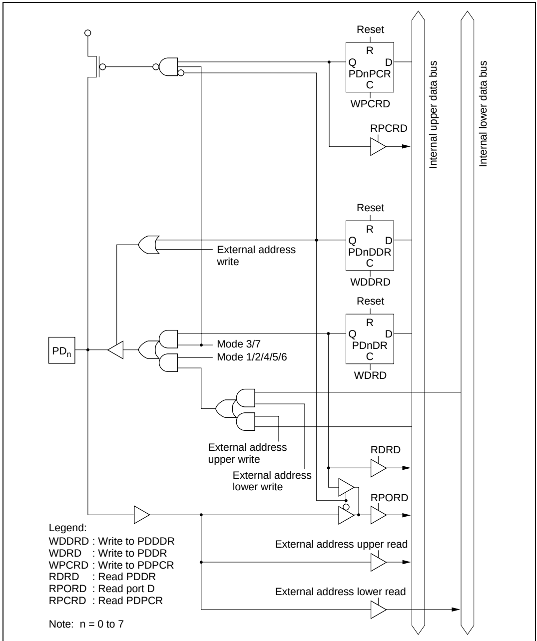
Figure C.8 Port D Block Diagram (Pin PD_n )
