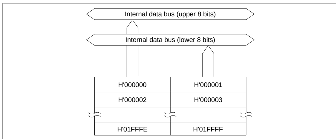
Figure 17.1 Block Diagram of ROM (H8S/2345)
