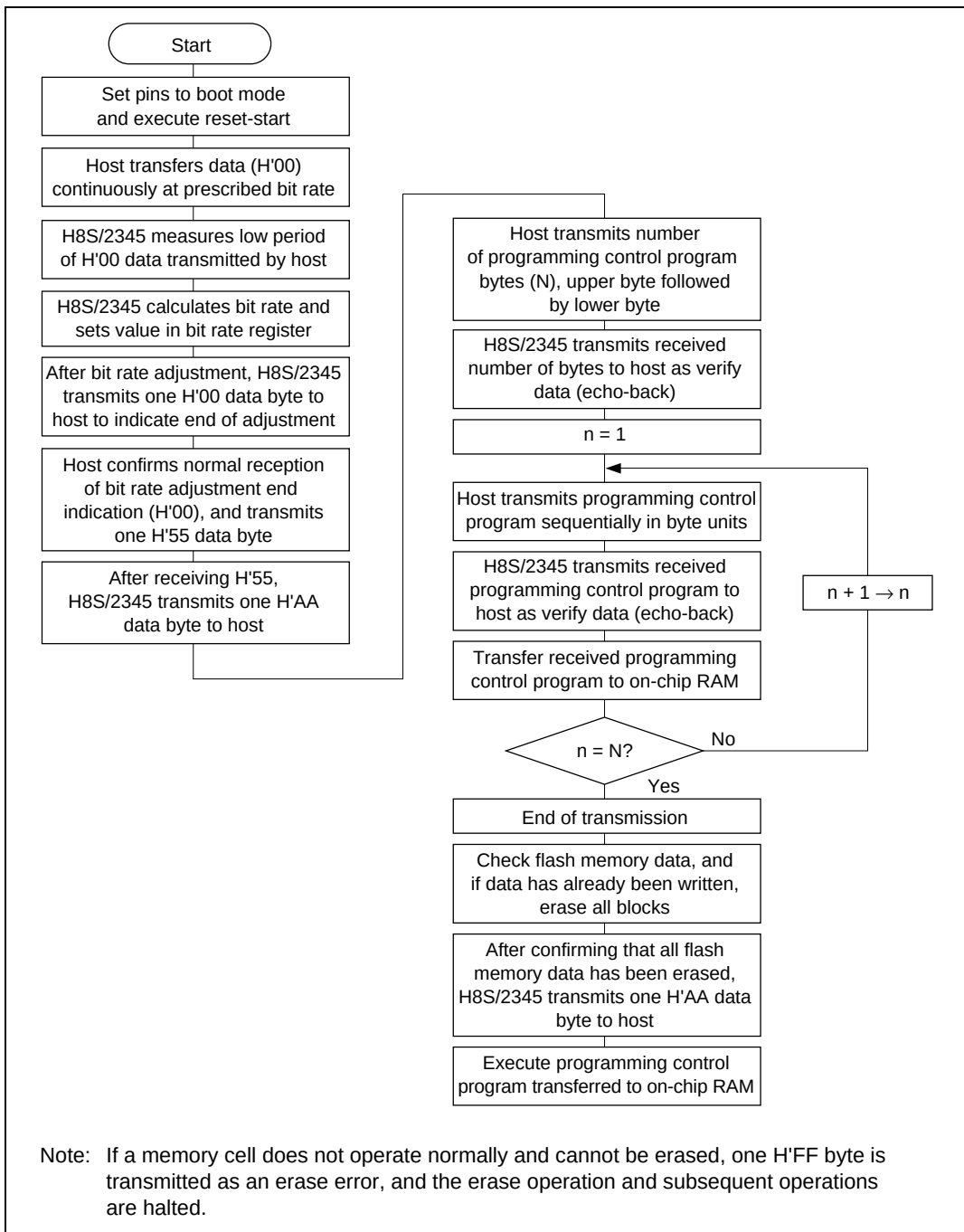
Figure 17.16 Boot Mode Execution Procedure
