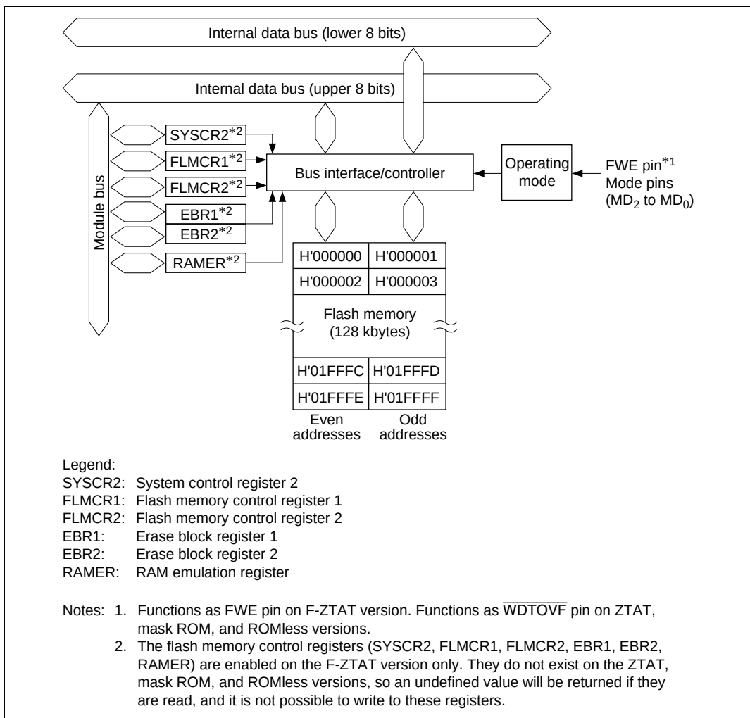
Figure 17.7 Block Diagram of Flash Memory
