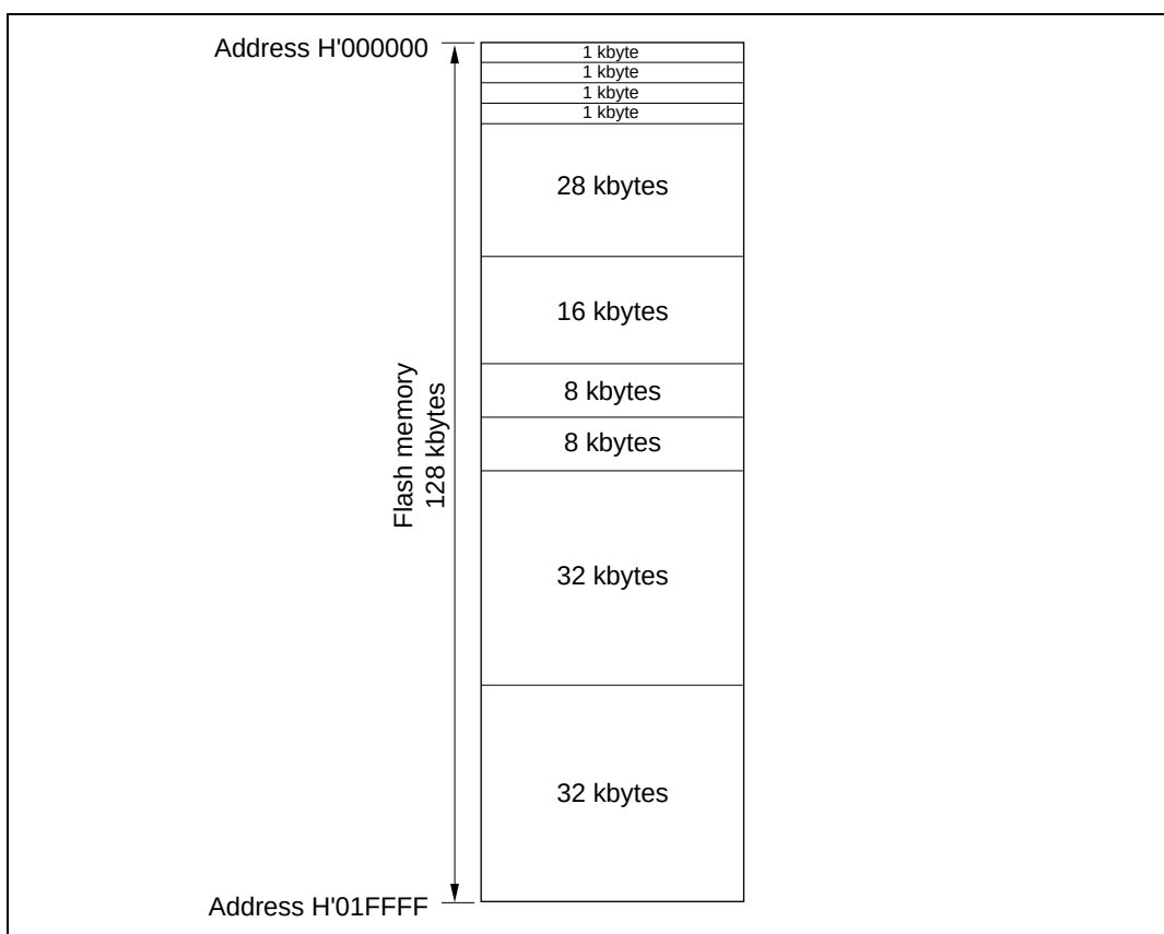
Figure 17.13 Flash Memory Block Configuration
