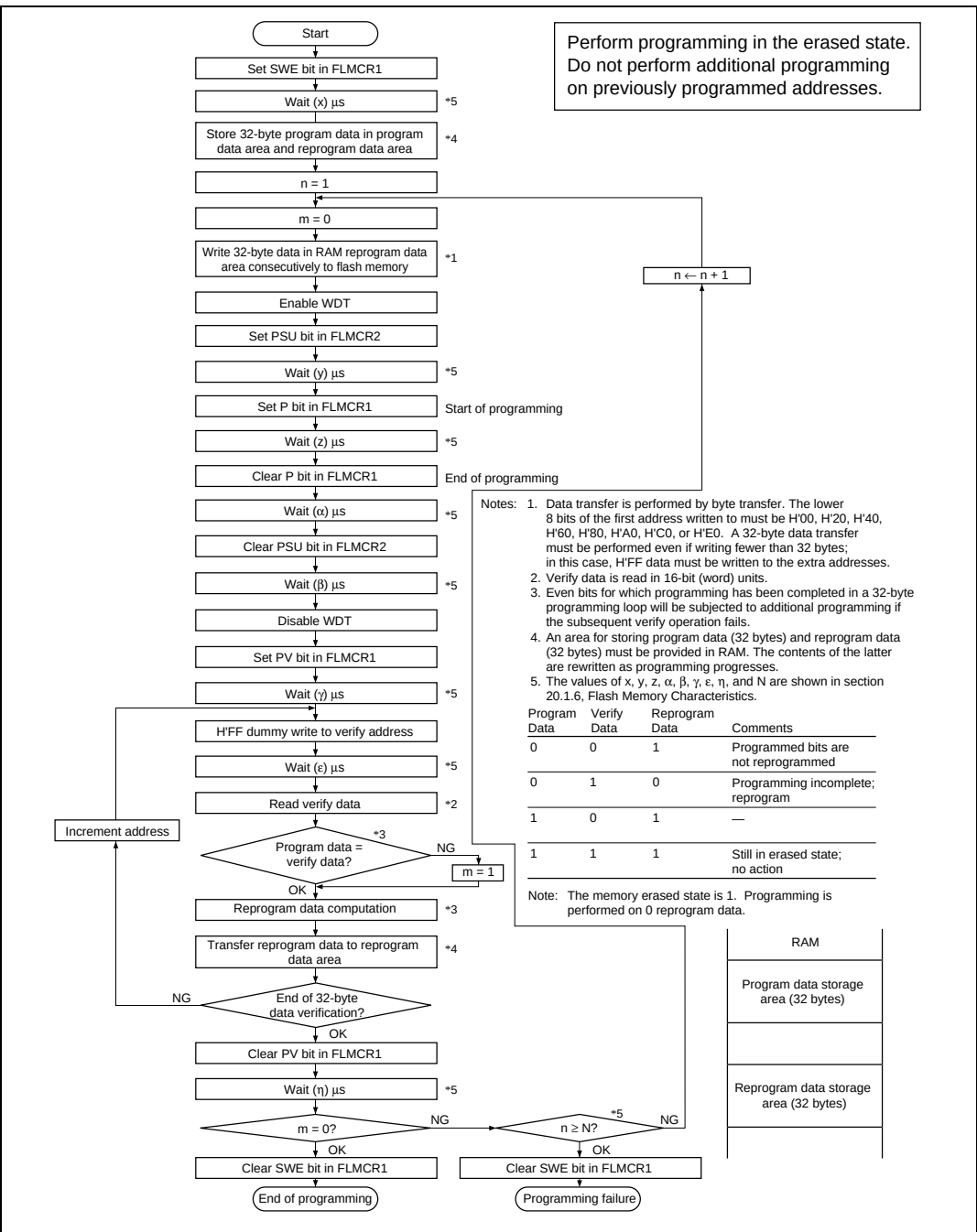
Figure 17.21 Program/Program-Verify Flowchart
