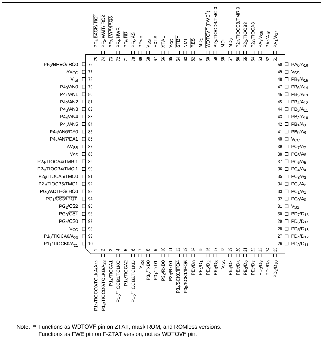
Figure 1.2 Pin Arrangement (FP-100B, TFP-100B, TFP-100G: Top View)
