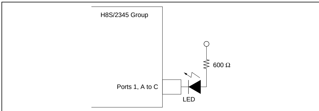
Figure 20.5 LED Drive Circuit (Example)
