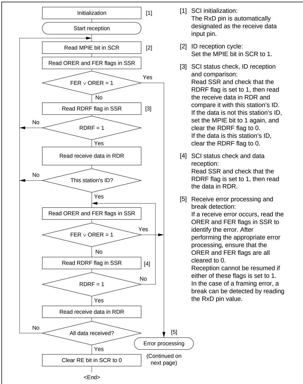
Figure 12.12 Sample Multiprocessor Serial Reception Flowchart
