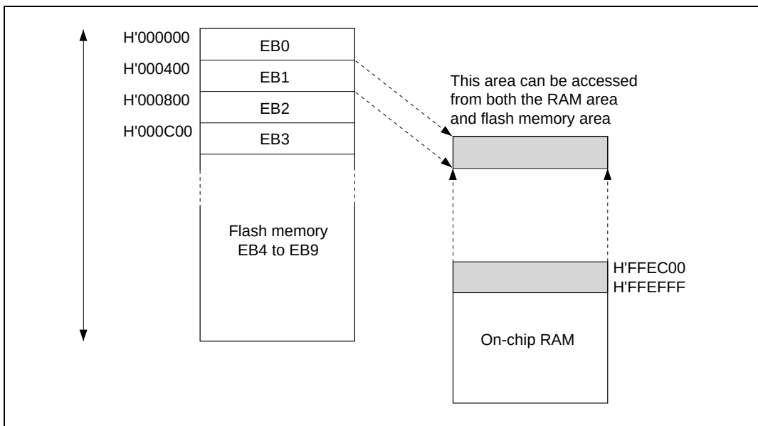
Figure 17.25 Example of RAM Overlap Operation
