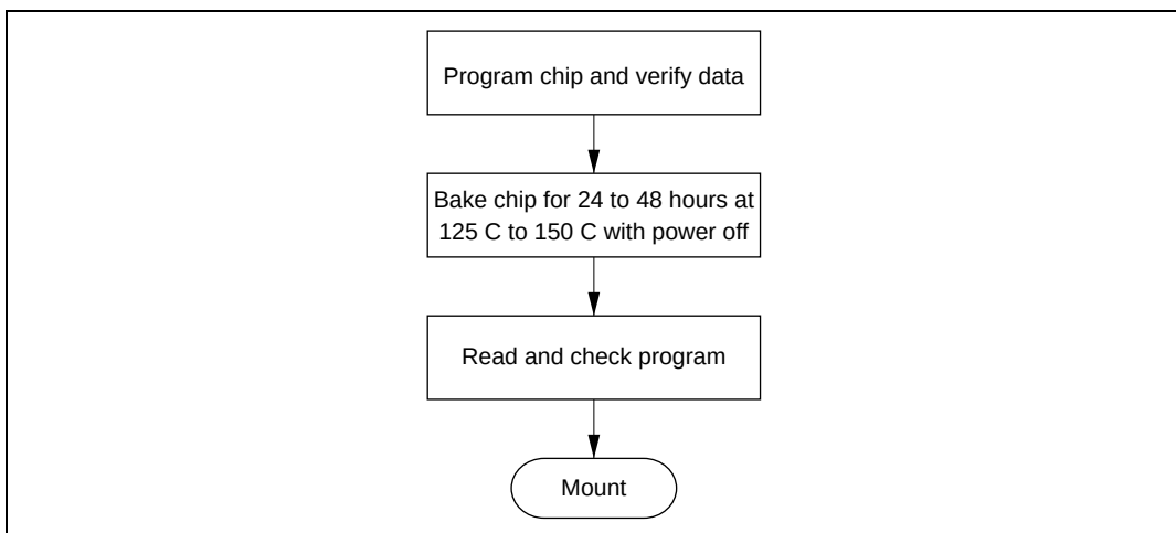
Figure 17.6 Recommended Screening Procedure
