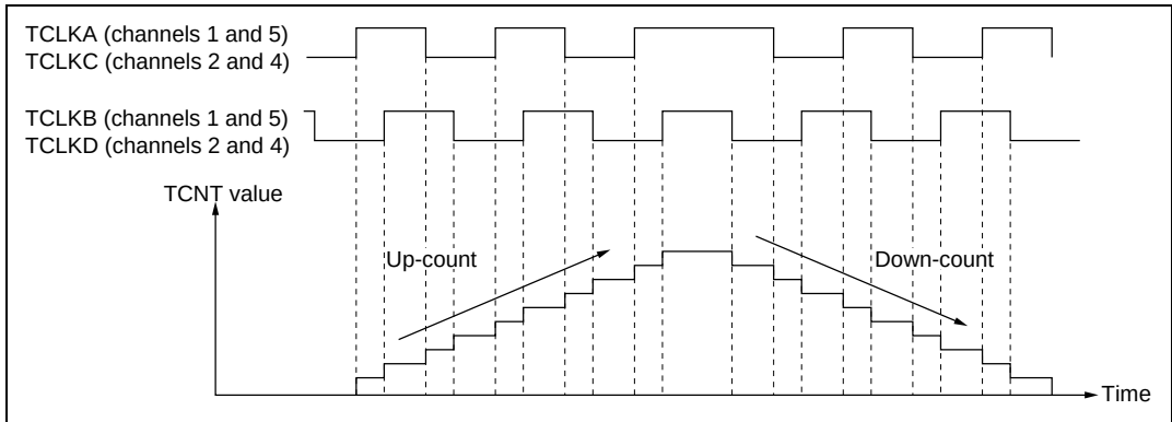
Figure 9.29 Example of Phase Counting Mode 1 Operation
