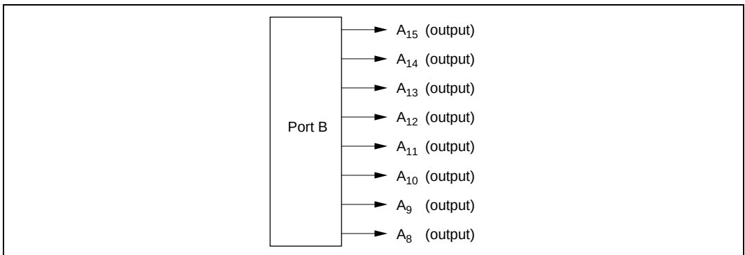
Figure 8.10 Port B Pin Functions (Modes 1, 4, and 5)*
