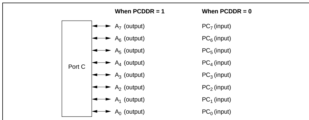
Figure 8.15 Port C Pin Functions (Modes 2 and 6)*
