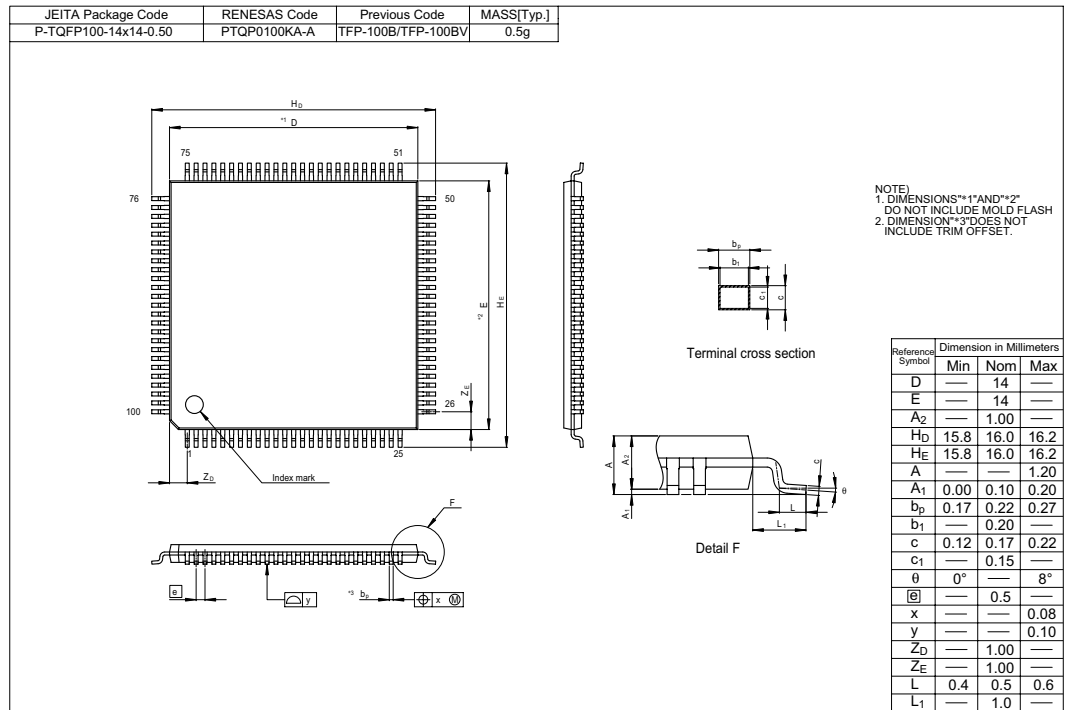
Figure G.1 TFP-100B Package Dimensions
