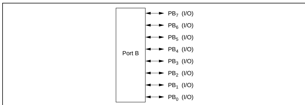
Figure 8.12 Port B Pin Functions (Modes 3 and 7)*
