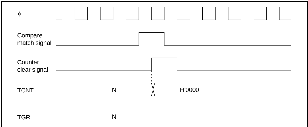
Figure 9.38 Counter Clear Timing (Compare Match)
