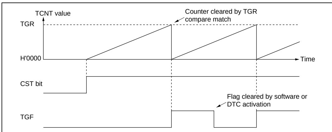
Figure 9.8 Periodic Counter Operation
