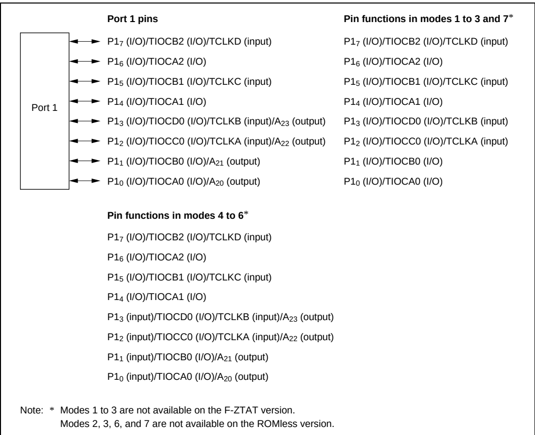
Figure 8.1 Port 1 Pin Functions
