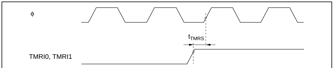
Figure 20.22 8-Bit Timer Reset Input Timing
