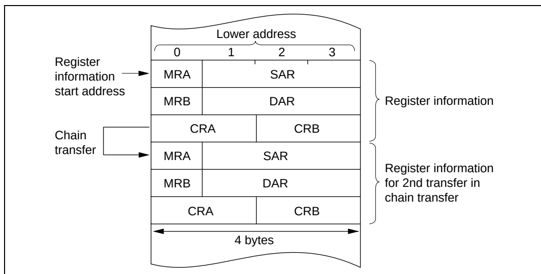
Figure 7.5 Location of Register Information in Address Space
