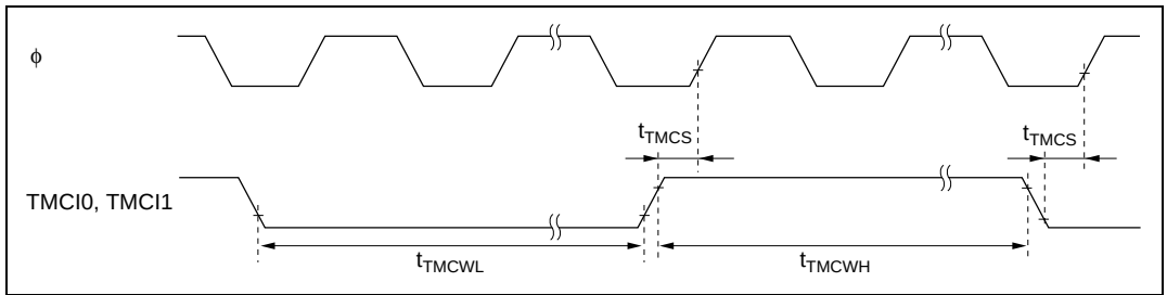
Figure 20.21 8-Bit Timer Clock Input Timing
