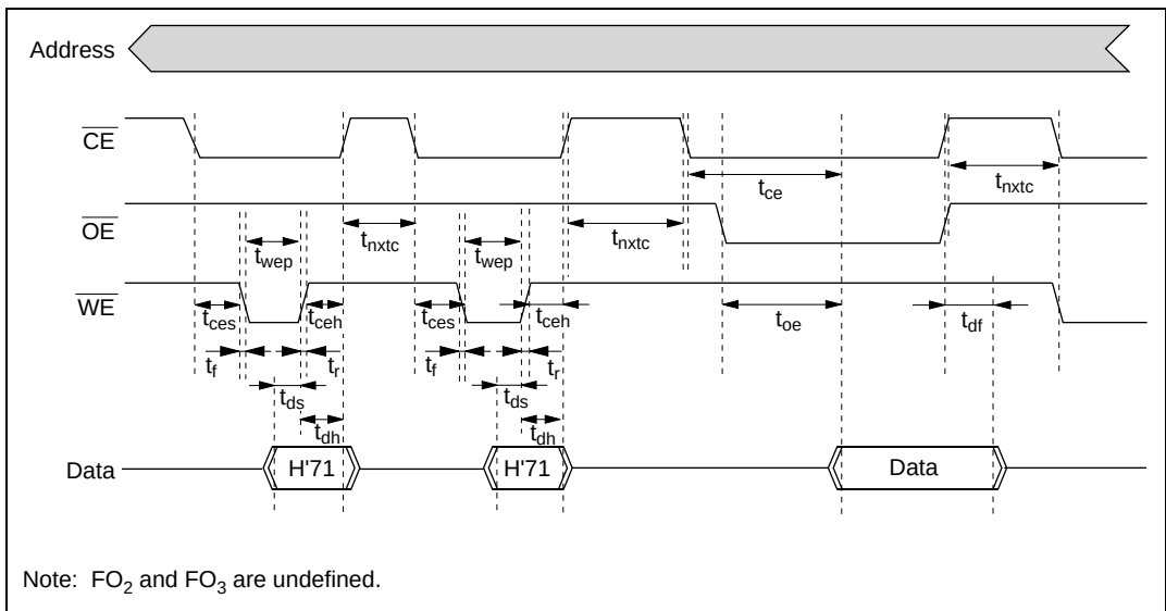
Figure 17.33 Status Read Mode Timing Waveforms
