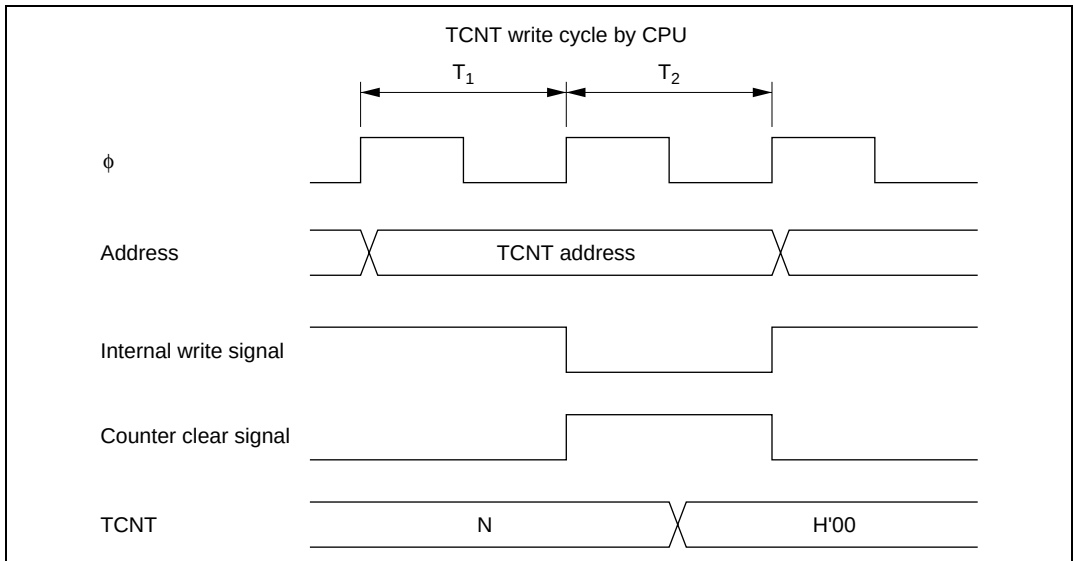
Figure 10.10 Contention between TCNT Write and Clear
