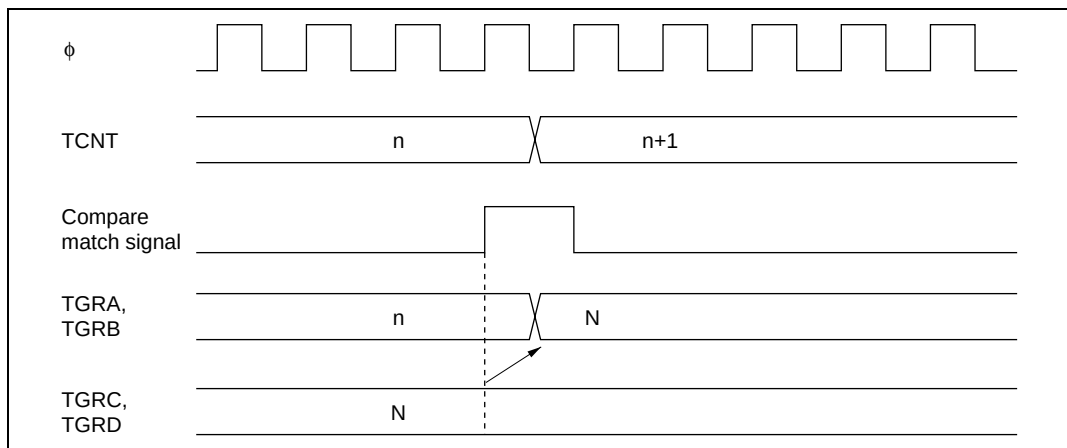
Figure 9.40 Buffer Operation Timing (Compare Match)
