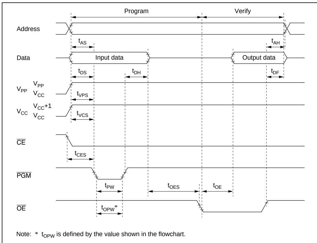
Figure 17.5 PROM Programming/Verification Timing
