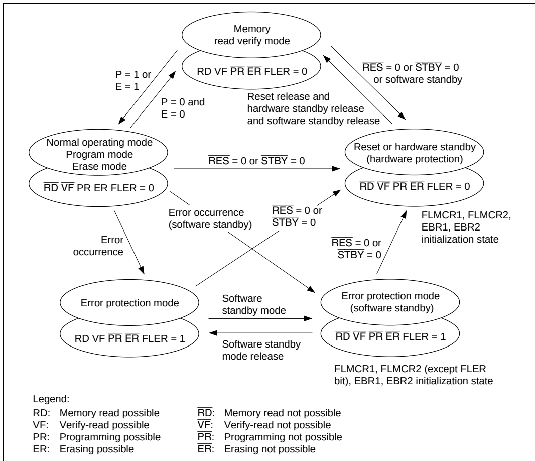
Figure 17.23 Flash Memory State Transitions
