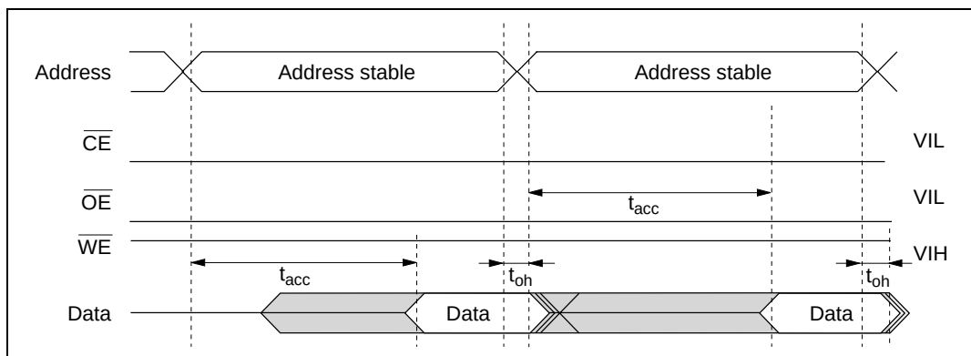
Figure 17.28 Timing Waveforms for \overline{\text{CE}}/\overline{\text{OE}} Enable State Read
