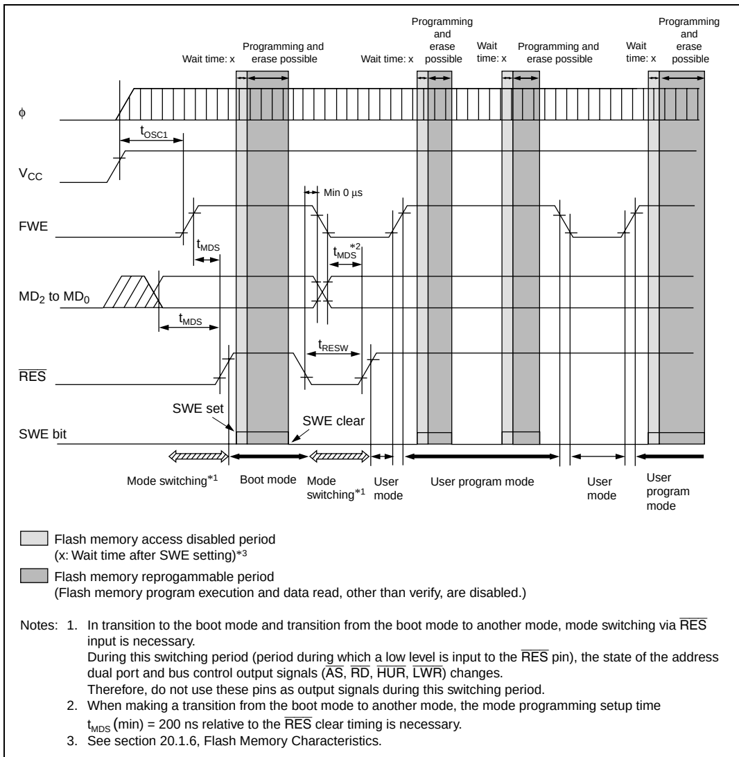
Figure 17.38 Mode Transition Timing (Example: Boot Mode → User Mode ↔ User Program Mode)
