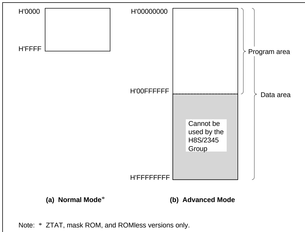
Figure 2.6 Memory Map
