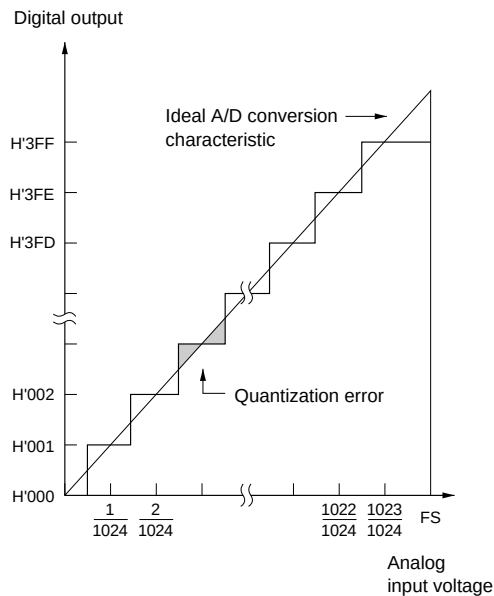
Figure 14.9 A/D Conversion Precision Definitions (1)
