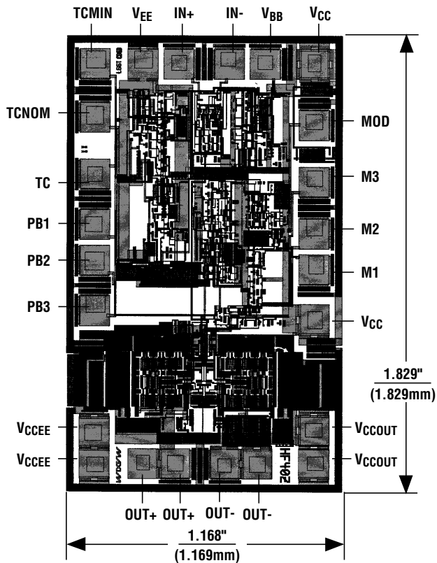
Chip Topography
