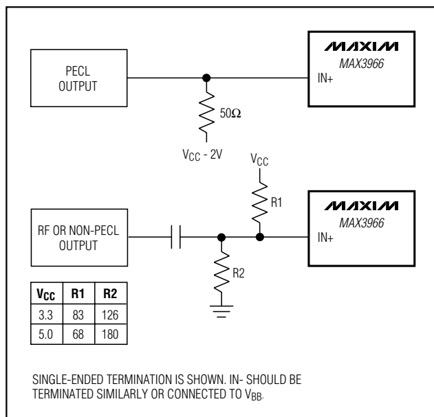
Figure 3. Input Terminations
